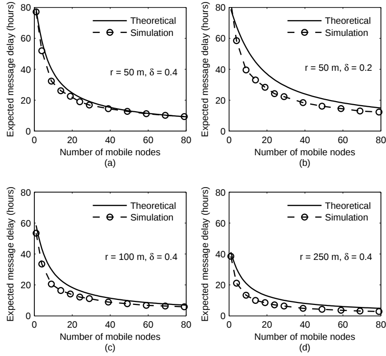
Figure 2.4: Message delay vs. number of nodes under the random walker mobility model.
