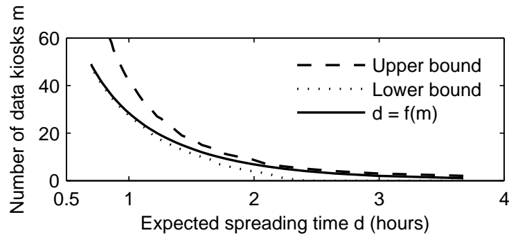
Figure 3.4: Bounds of the number of data kiosks and the function of expected spreading time.
