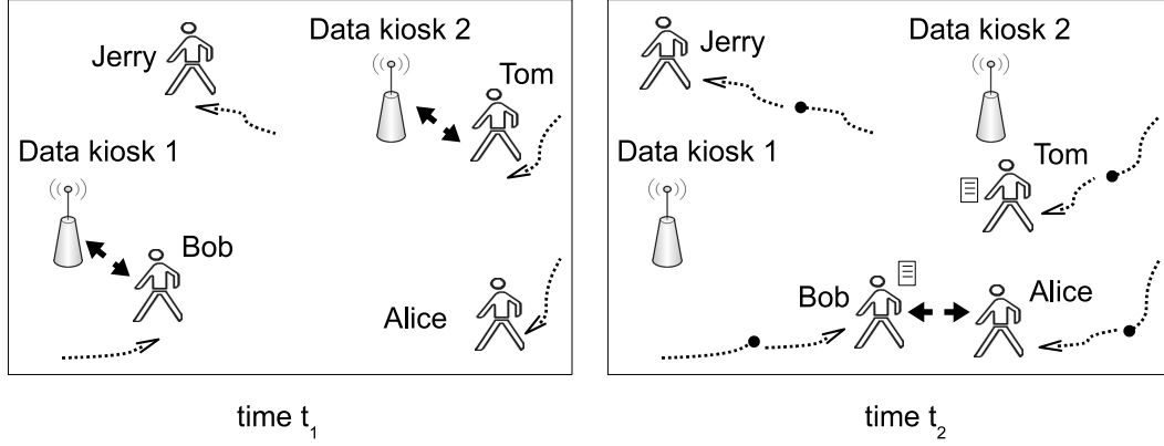
Figure 1.2: Content distribution in infrastructure-dependent DTNs.
