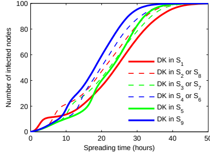
Figure 4.6: Numerical solutions in a case of a system of nine regions.
