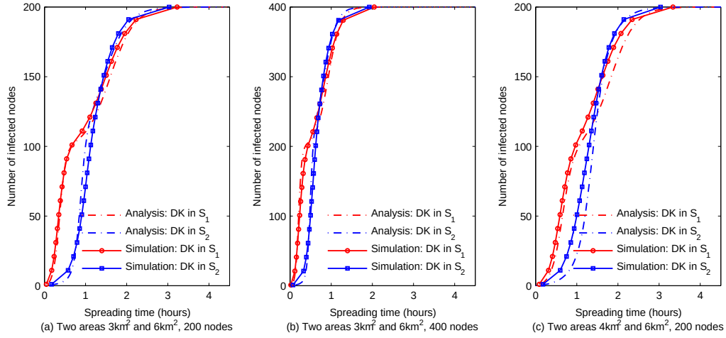
Figure 4.8: Number of infected nodes for different number of mobile nodes and inter-contact times.
