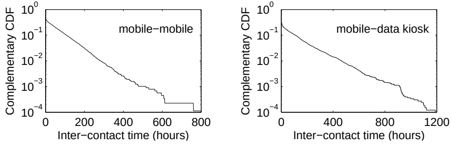
Figure 3.2: CCDF of inter-contact time for the random walker mobility model.
