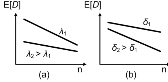
Figure 2.1: Asymptotic representation of the expected message delay.
