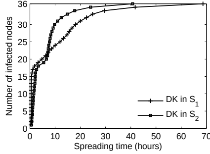
Figure 4.10: The evolution of infected nodes in an area of two regions using real-world traces.
