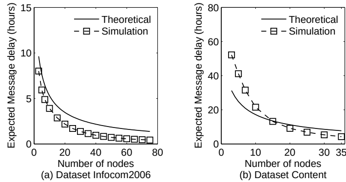
Figure 2.8: Expected message delay on the experiment data.
