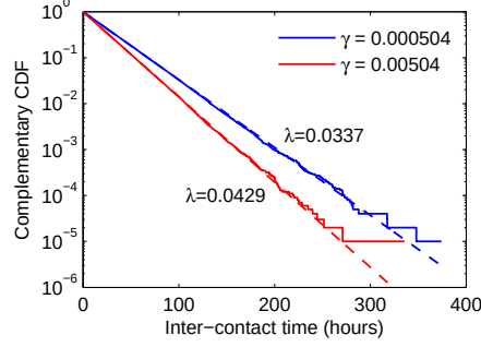
Figure 4.7: CCDF of inter-contact times for different moving rates.
