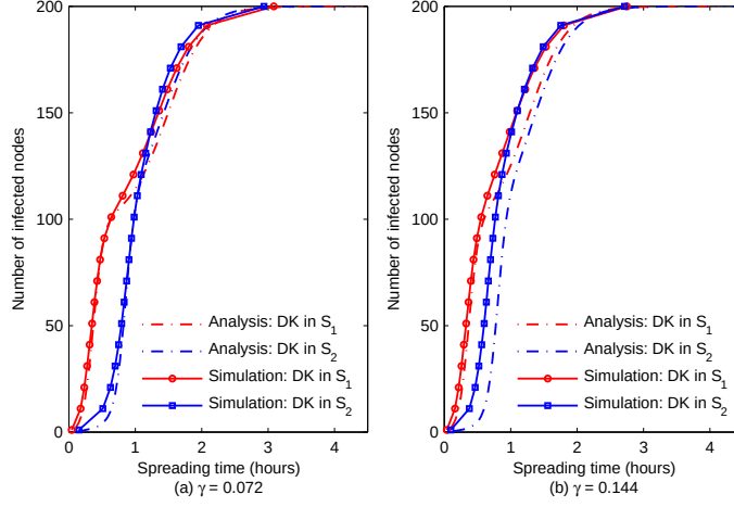
Figure 4.9: Number of infected nodes for different moving rates.
