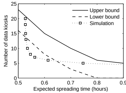
Figure 3.5: Number of data kiosks vs. expected spreading time for dataset Infocom2006.
