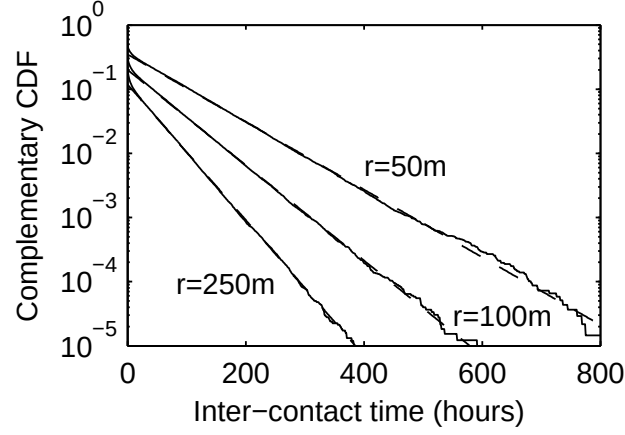
Figure 2.2: CCDF of inter-contact time for random walker.
