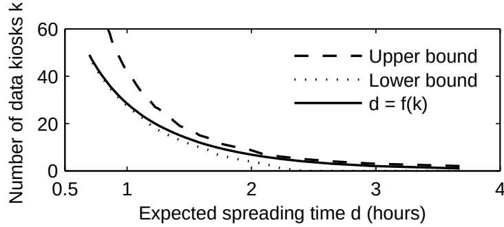
Figure 3.4: Bounds of the number of data kiosks and the function of expected spreading time.
