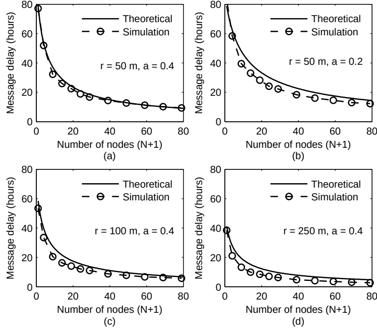
Figure 2.4: Message delay vs. number of nodes under the random walker mobility model.
