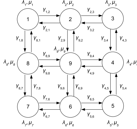
Figure 4.5: The parameters of a system of nine regions.
