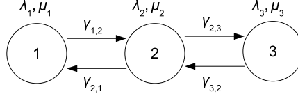
Figure 4.2: The parameters of a system of three regions.
