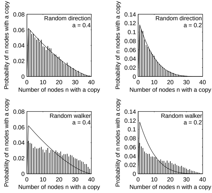
Figure 2.5: Distribution of the number of copies: r=50m .
