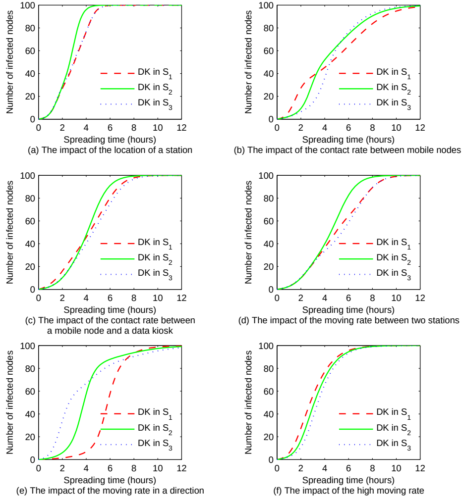
Figure 4.3: Placing one data kiosk in an area of three regions.
