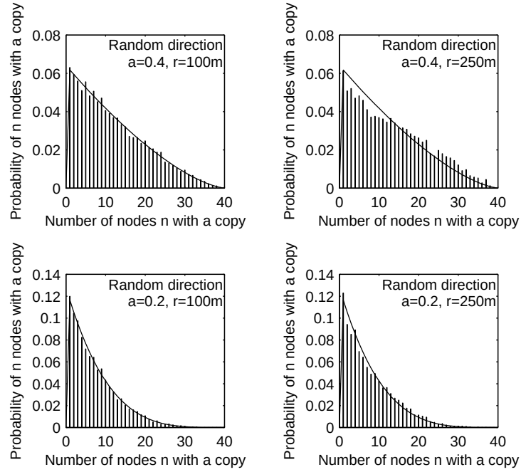
Figure 2.6: Distribution of the number of copies: r=100m , 250m .
