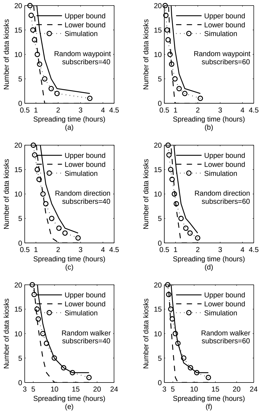
Figure 3.3: Number of data kiosks vs. spreading time.
