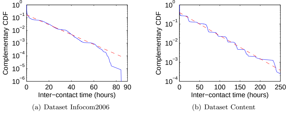
Figure 2.7: CCDF of the inter-contact time in dataset Infocom2006 and Content.
