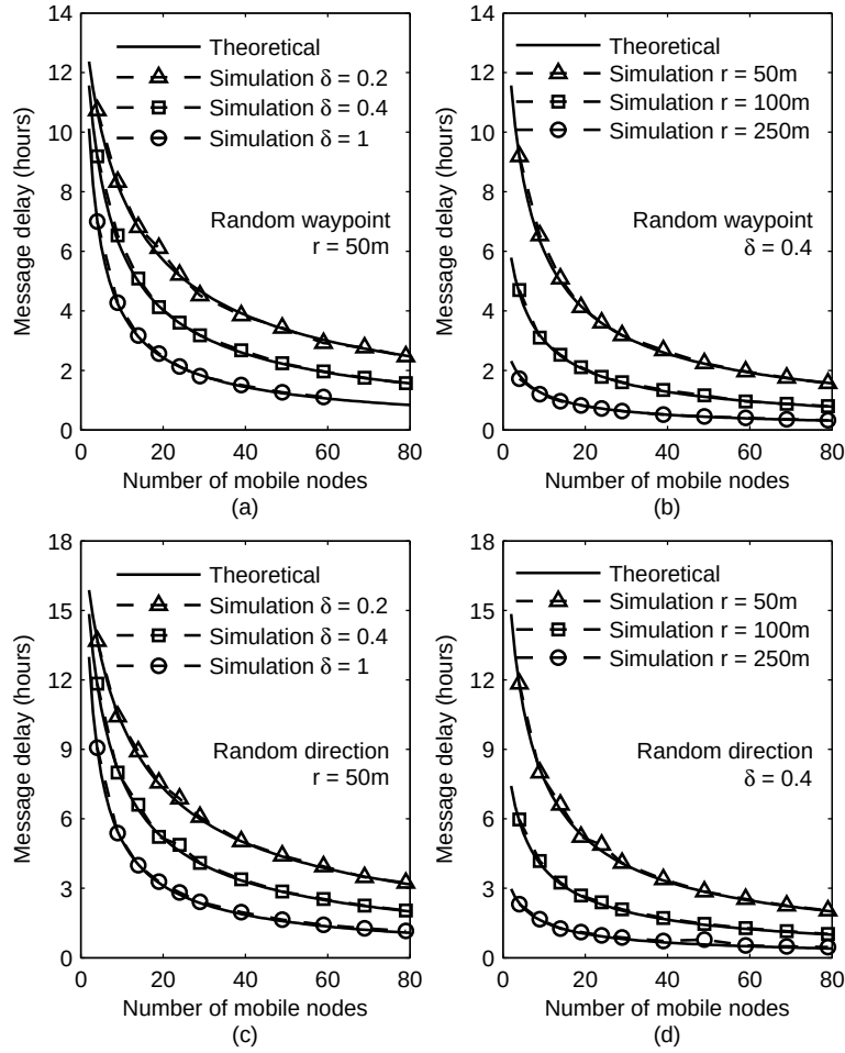
Figure 2.3: Message delay vs. number of nodes under the random waypoint and random direction mobility model.
