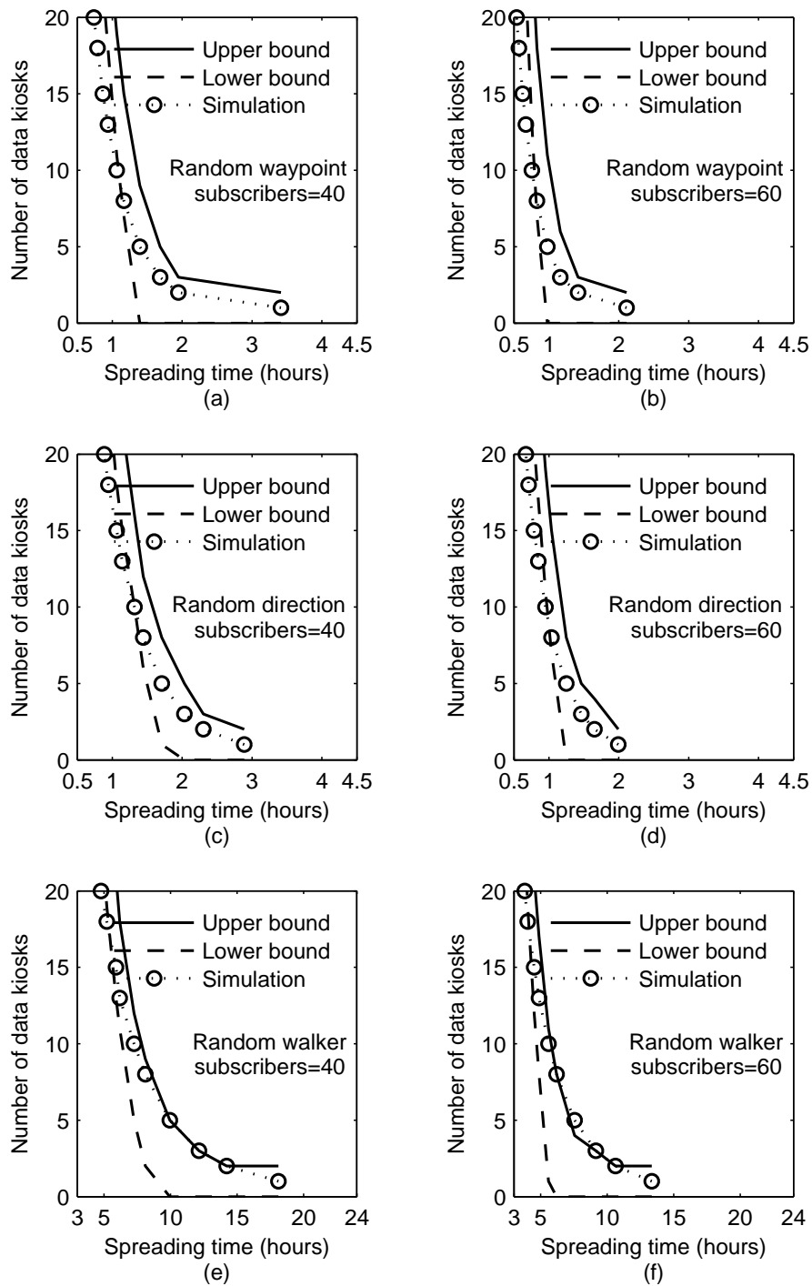
Figure 3.3: Number of data kiosks vs. spreading time.
