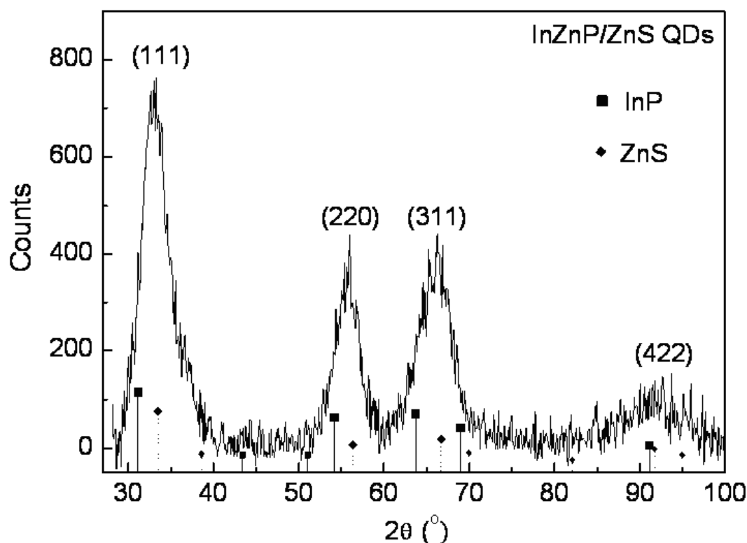
Figure 4.6: XRD pattern of In(Zn)P/ZnS NCs synthesized with the \text{Zn}^{2+}:\text{In}^{3+} molar ratio of 1:1, the reaction-growth temperature for forming the core and the shelling temperature were fixed at 300°C and 285°C respectively, and the shelling time was 1 hr. The diffraction patterns corresponding to pure bulk InP and ZnS are also indicated for comparison.
