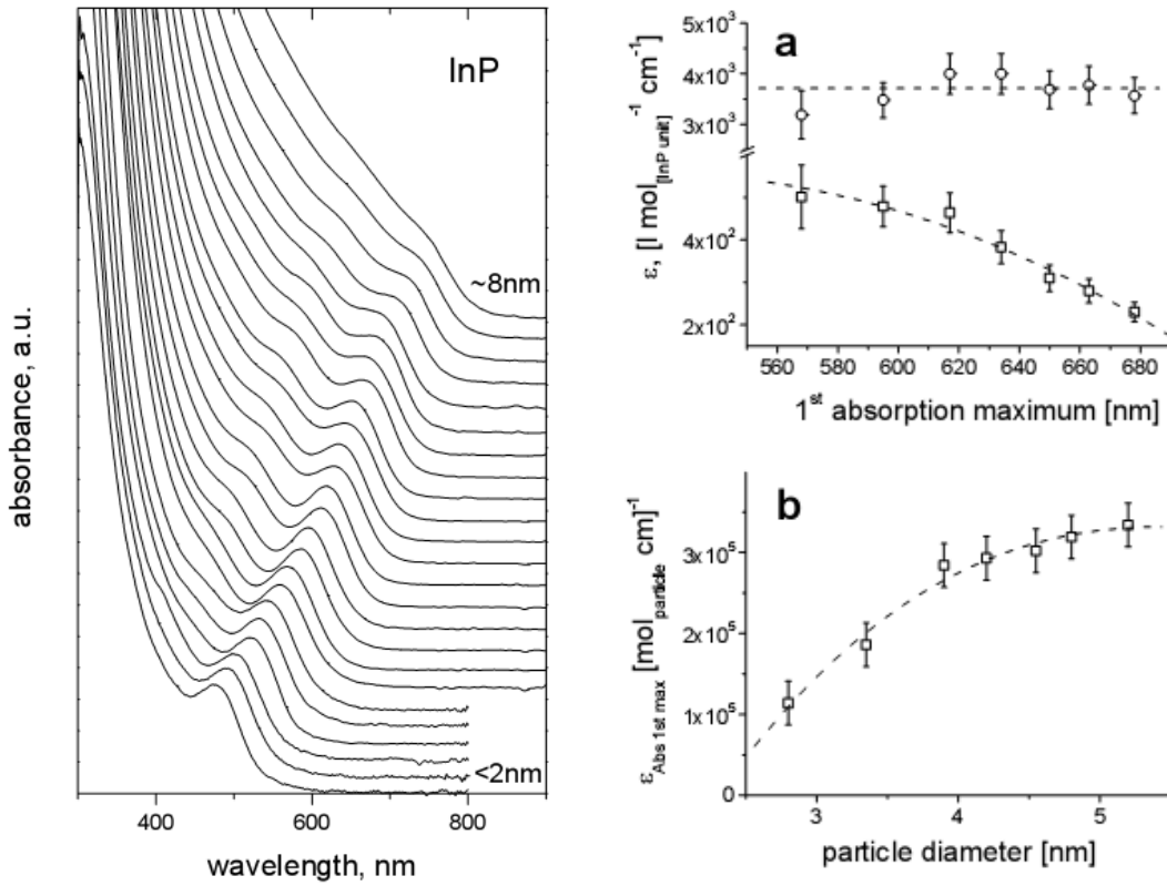
Size-dependent evolution of absorption spectra of TOPO-TOP capped InP NCs (left). (a) the extinction coefficients referred to the concentration of InP units measured at 350 nm ( \square ) and at the first absorption maximum ( \square ) for different nanocrystal sizes; (b) molar extinction coefficient of InP nanocrystals at the first absorption maximum referred to the particle concentration [11].
