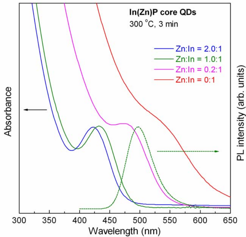
Figure 4.9: Absorption spectra of In(Zn)P core only QDs synthesized at 300°C for 3 min as a function of the \text{Zn}^{2+}:\text{In}^{3+} molar ratio. A typical PL of In(Zn)P core QDs with the \text{Zn}^{2+}:\text{In}^{3+} molar ratio of 1:1 is also presented (dashed line).
