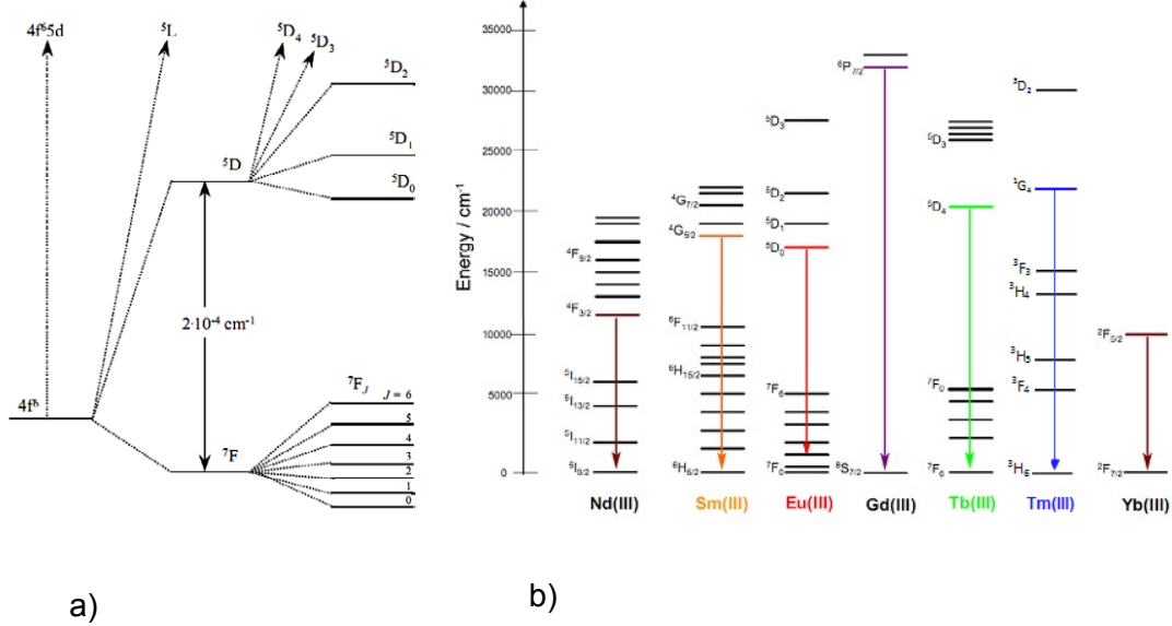
Figure 2.3: (a) energy levels of \text{Eu}^{3+} ions and (b) partial energy diagram of selected \text{RE}^{3+} ions. Arrows show the main transitions [28].
