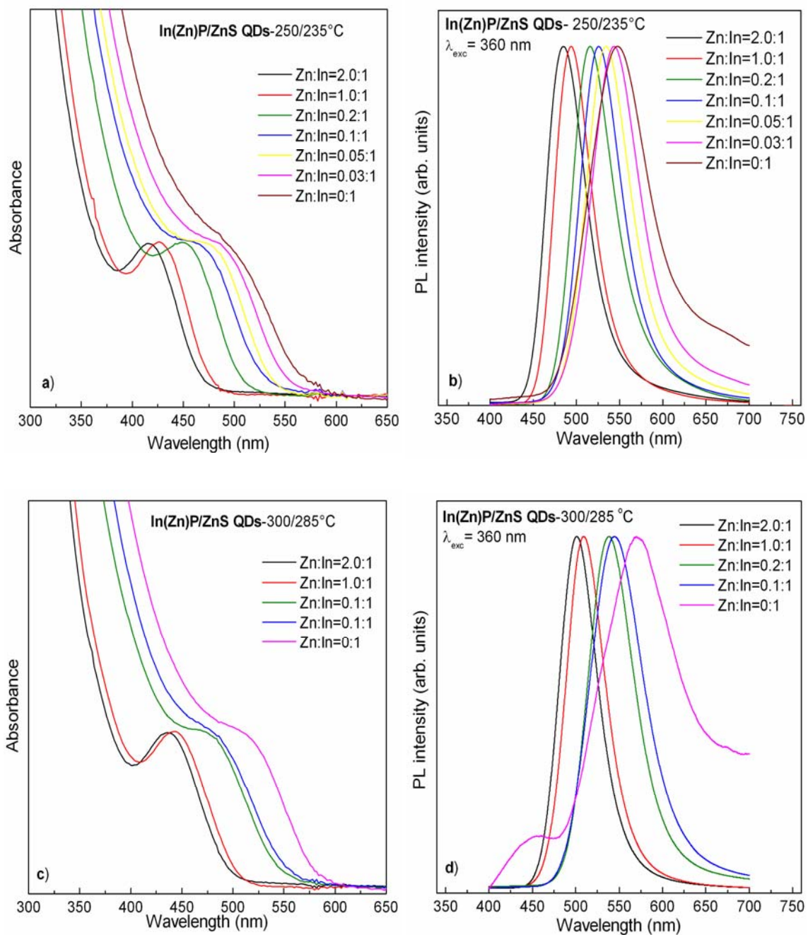
Figure 4.10: Absorption (a, c) and PL (b, d) spectra of In(Zn)P/ZnS QDs as a function of the \text{Zn}^{2+}:\text{In}^{3+} molar ratio and the reaction-growth/shelling temperatures (indicated on the figures).
