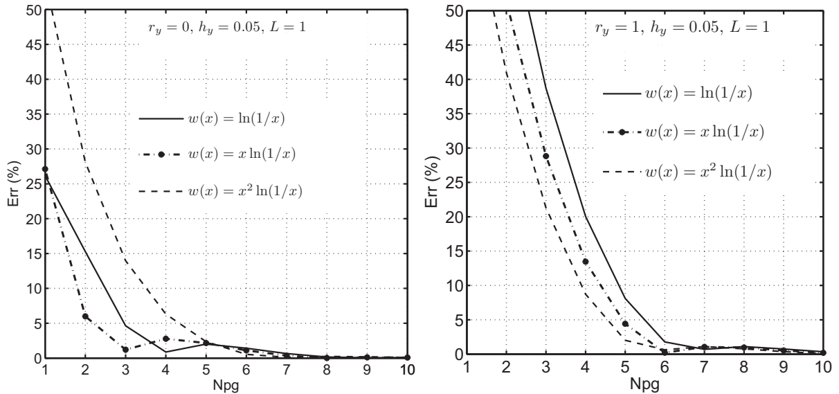
Figure 4.8 : Convergence Gauss-Log
