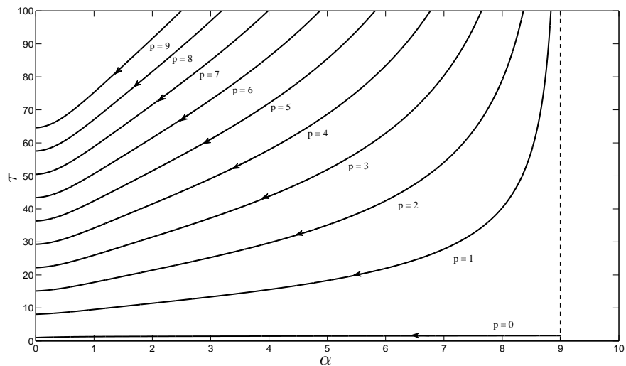
Figure 5.2: Example 5.1: T_1^p for p = 0, \dots, 9 (type 3/2).
