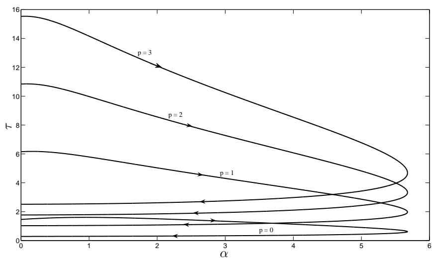
Figure 5.3: Example 5.1: T_2^p for p = 0, 1, 2, 3 (type 2/2).
