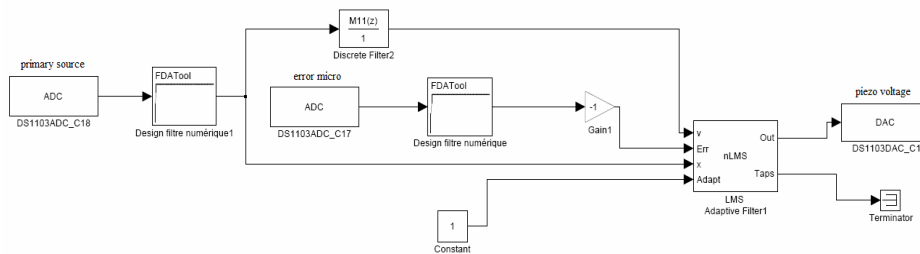
Fig.5-12 The configuration of the active control
