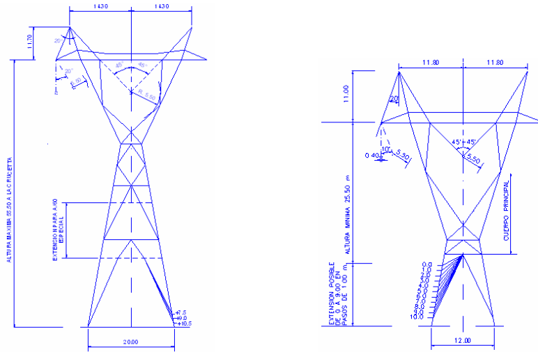
d) A/60 angle tension tower 27 ton
