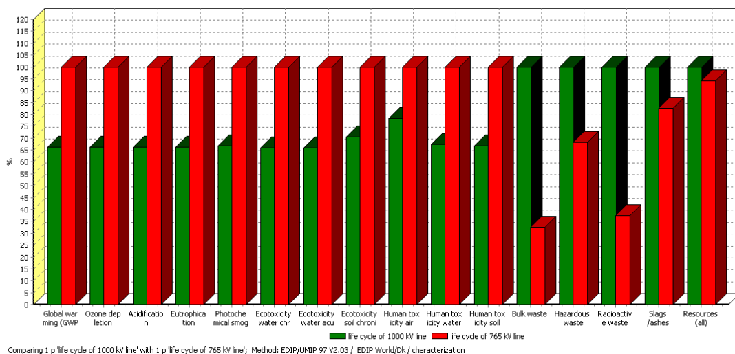
Fig. 4-4 : Environmental impacts comparison between 1000 kV and 765 kV AC transmission line (by coal-generated method)
