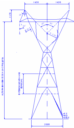
d) A/60 angle tension tower 27 ton
