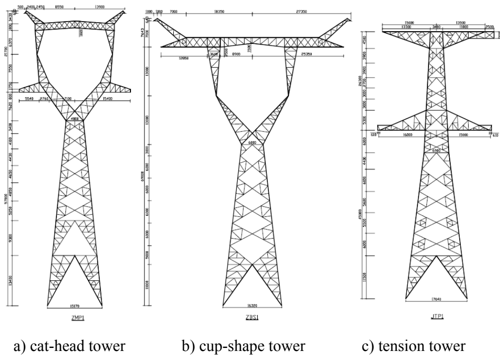
Fig. 4- 2 : Tower types in 1000 kV AC project [69]
