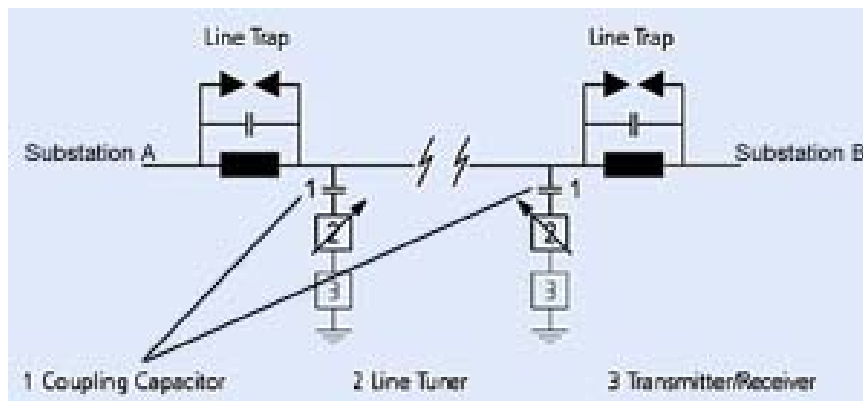
Fig. 3-39 : Illustration of lines traps and coupling capacitor
