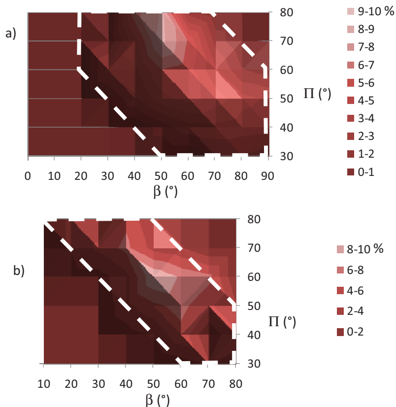
FIG. IV.27 - Distribution of angles \beta and \Pi of a) slip system with the highest Schmid factor and b) initiated PSB cracks.
