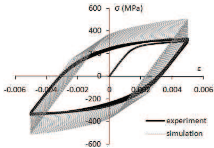
FIG. III.11 - Simulation of the first 20 cycles of a tension-compression test with \epsilon = 0.5\% using the CP localization law.
