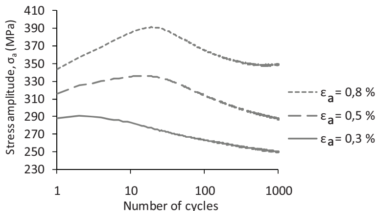
FIG. II.6 - Cyclic hardening/softening curves in semi-log diagram.
