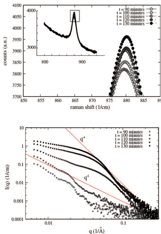
Figure 2. Raman spectra and small-angle X-ray scattered intensity as a function of time for the sample prepared with 20 mM of L-arginine and T = 70\text{ }^\circ\text{C} .
