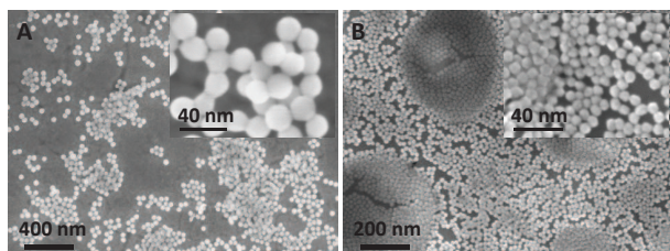
Figure 3: Comparison of the final particles obtained at different stirring rates ( T=65^\circ\text{C} , catalyst: arginine 6mM). A: stirring 250rpm (diameter 40.4nm, PDI 1.024), B: stirring 1000rpm (diameter 18.2nm, PDI=1.029)
