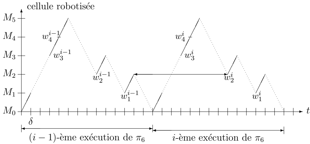
Figure B.2: La permutation pyramidale \pi_6 = (A_0 A_3 A_4 A_2 A_1)
