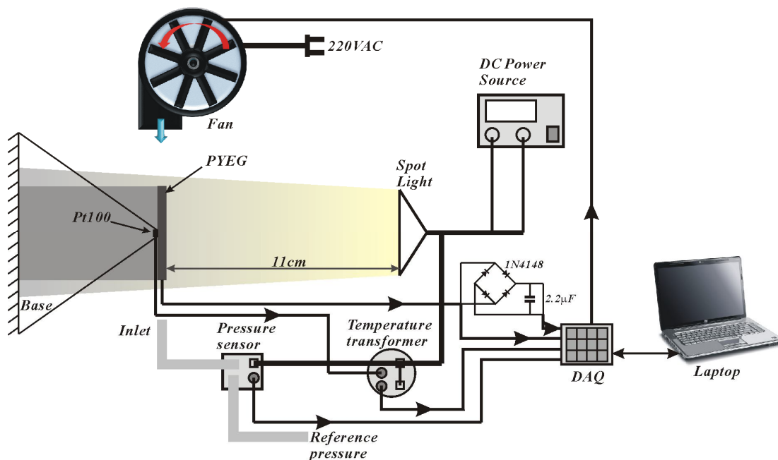
Figure 5. 3: Diagram of experiment system of solar PYEG in lab
