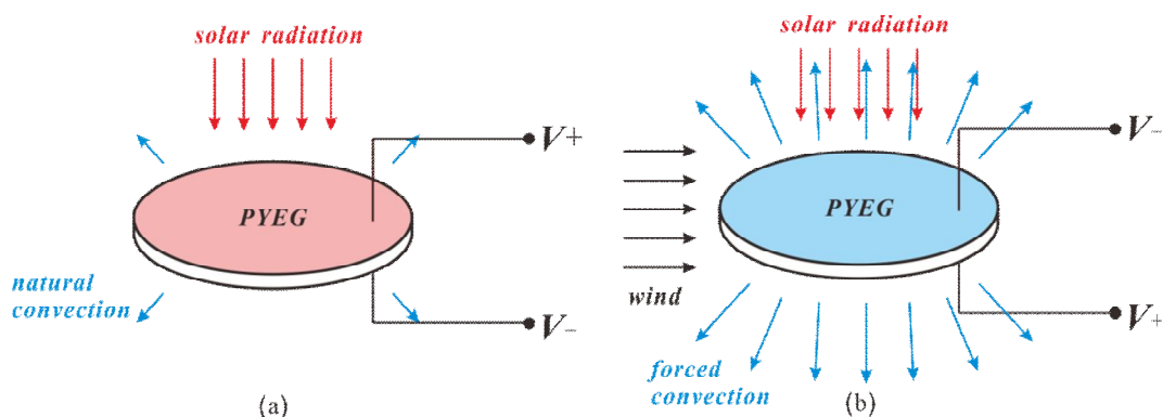
Figure 5. 1: Principle of solar energy harvesting with PYEG and wind: (a) temperature increases with weak natural convection (b) temperature decreases with strong forced convection
