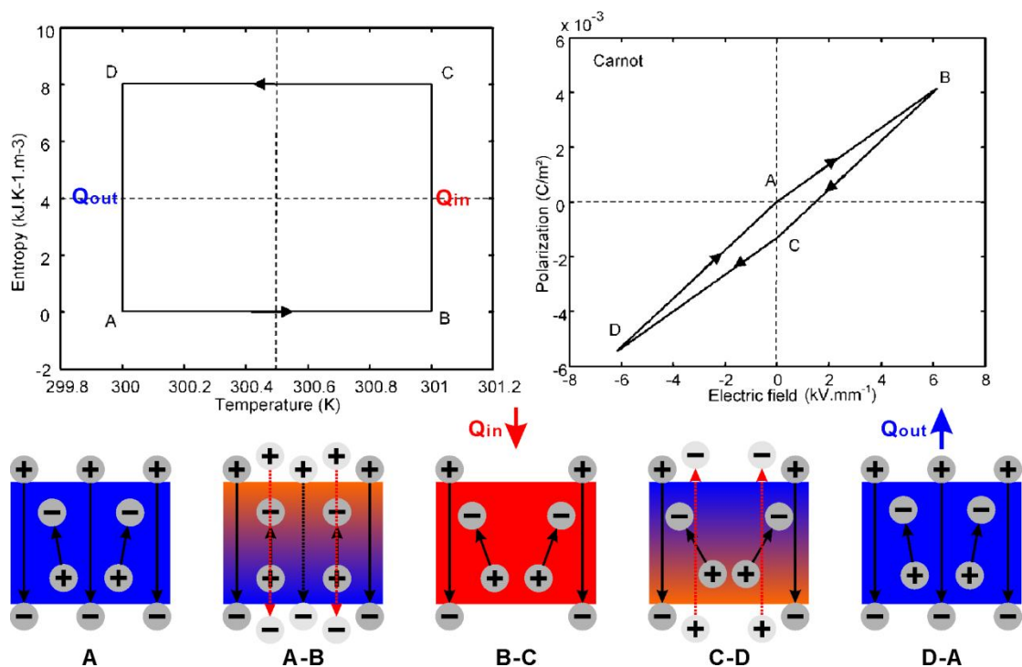
Figure 2. 10: Pyroelectric energy conversion process by Carnot cycle [SEB 2008]
