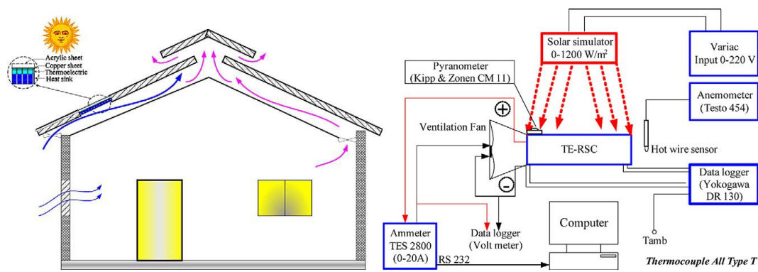
Figure 3. 4: Solar TEG as indoor ventilation [MAN 2004]
