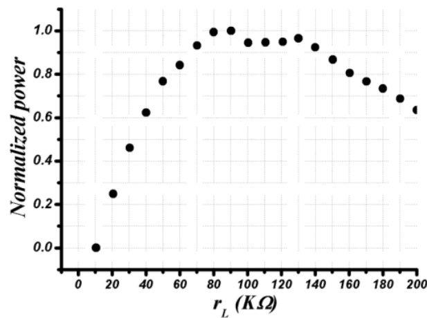
Figure 6. 4: Power generation with different external resistor
