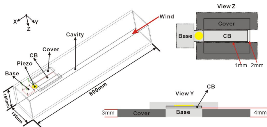
Figure 6. 2: Prototype piezoelectric energy harvesting system
