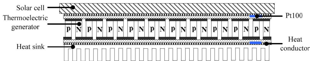
Figure 3. 6: PV and TEG hybrid system [SHA 2007]
