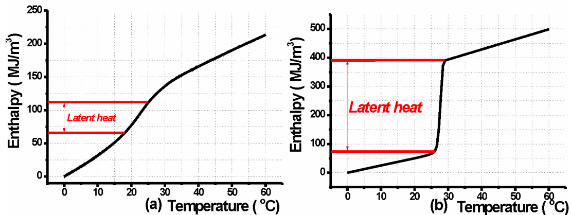
Figure 4. 7: Enthalpy of PCM as a function of temperature: (a) paraffin wax (b) salt hydrates
