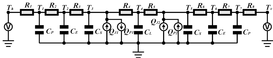
Figure 4. 14: Full electric model of the TEG
