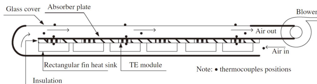
Figure 3. 5: Diagram of double-pass thermoelectric solar air collector [LER 2008]
