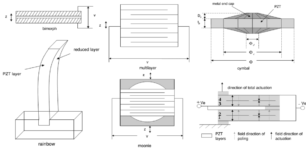
Figure 2. 16: Common modes of mechanical coupling structure of piezoelectric element [WEB 1999]
