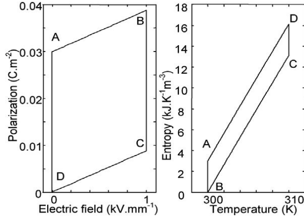
Figure 2. 11: Pyroelectric energy conversion process by Ericsson cycle [SEB2 2008]
