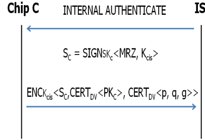
Figure 5.3: e-Passport Authentication
