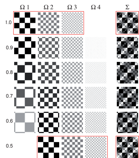
Figure 2.14: “Dynamic Canvas” infinite zoom mechanism applied on a checkerboard texture. For each zoom factor (left) the four octaves as well as their weighted sum is shown. From [CTP*03].
