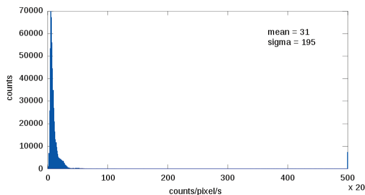
FIGURE 4.16: Histograms of the pixel counts (a) in a flat image and (b) in an image of the pocket watch obtained with a 50 ms pose.
