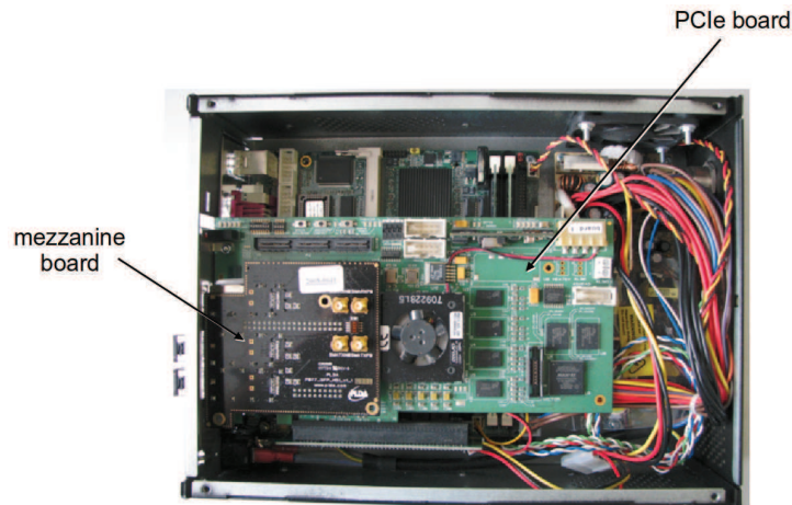
FIGURE 3.29: Picture of the PCI Express board plugged to the acquisition PC with its mezzanine daughter board containing optical transceivers.
