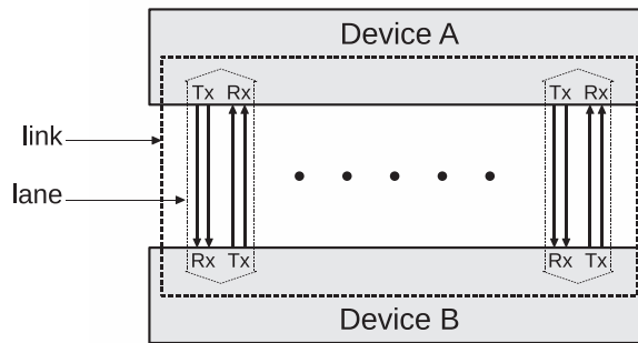
FIGURE 3.31: Scheme of a PCI Express link.
