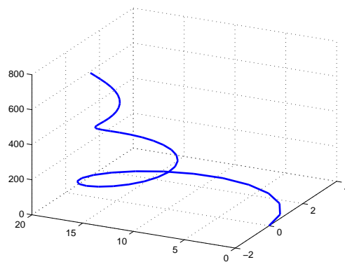
FIGURE 3.3: Illustration of \Delta(\epsilon_k) : system matrix with complex-conjugated eigenvalues.
