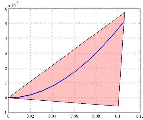
FIGURE 3.1: Illustration of the containment of \Delta(\epsilon_k) by a simplex: non-defective system matrix with real eigenvalues.
