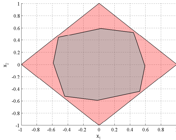
FIGURE 7.4: Set \mathcal{P} and set iterate A_0\mathcal{P} \oplus A_1\mathcal{P} .
