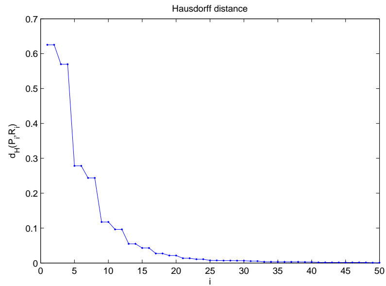
FIGURE 7.12: d_H(\mathcal{R}_i, \mathcal{P}_i) vs. the iteration index i .
