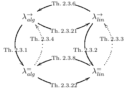
A \rightarrow B means “ A is simulated by B ”
