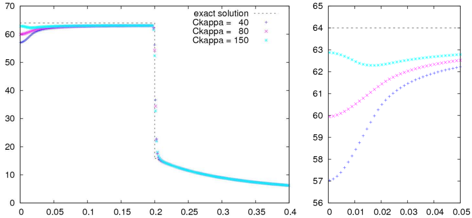
Figure 6.7: Density along the z = r axis for the two-dimensional Noh problem at time t = 0.6 on 400 cells with different values of C_\kappa : whole computational domain (left) and zoom on the [0; 0.05] region (right).
