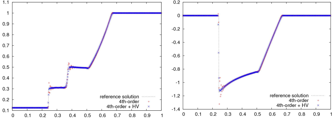
Figure 6.1: One-dimensional Sod shock tube in cylindrically symmetric geometry at time t = 0.14 . Density (left) and velocity (right) obtained on 400 cells with the fourth-order scheme. The reference solution has been obtained using a first-order accurate Lagrange-remap scheme cylindrical geometry [30] on 100,000 cells.
