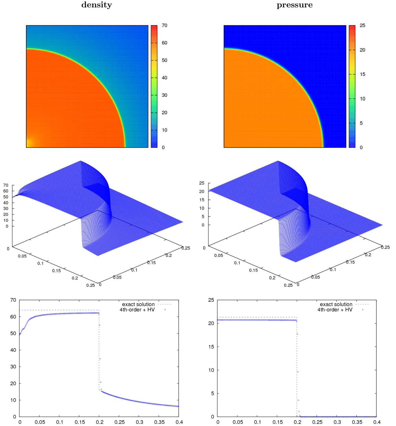
Figure 6.5: Two-dimensional Noh problem in spherically symmetric geometry: density (left) and pressure (right) obtained at time t = 0.6 . From top to bottom: map plot, surface plot and slice along the z = r axis.
