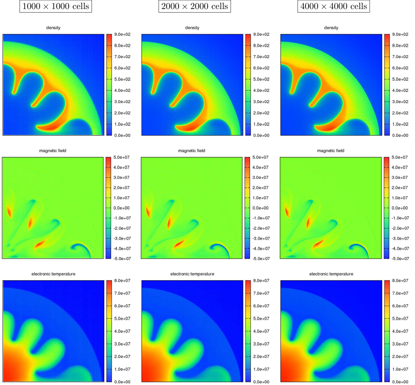
Figure 8.10: Numerical results to the two-temperature ICF test problem with A_0 = 5 \cdot 10^{-4} cm at time t = 600 ps on 1000 \times 1000 , 2000 \times 2000 and 4000 \times 4000 cells (zoom on the [0; 0.008]^2 square). From top to bottom: density, magnetic field and electronic temperature.
