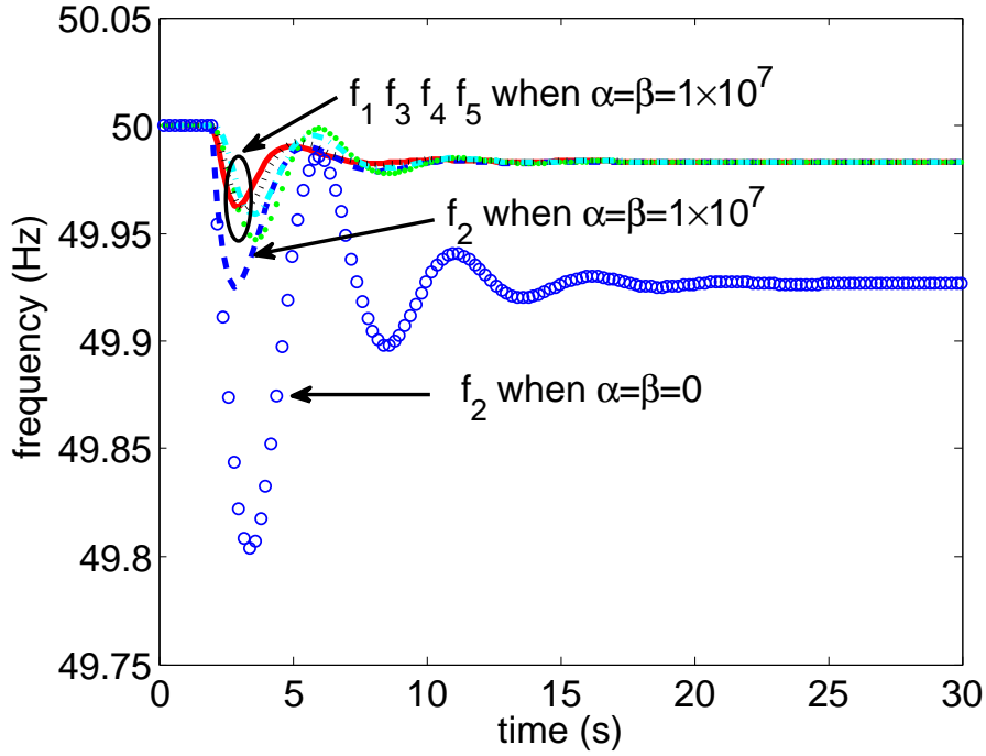
Figure 5.3: Frequencies of the five AC areas under the power-injection-based control scheme when \tau = 0\text{s} and \alpha = \beta = 1 \times 10^7 . The evolution of f_2 when \alpha = \beta = 0 is also shown.
