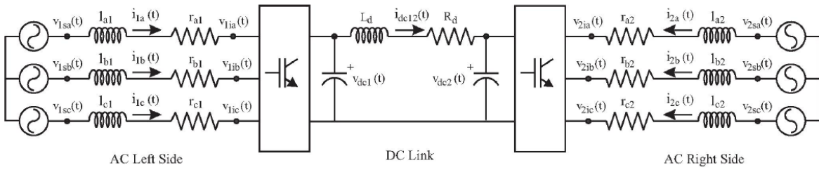
Figure 3.8: Three-phase diagram of a VSC-base HVDC link.
