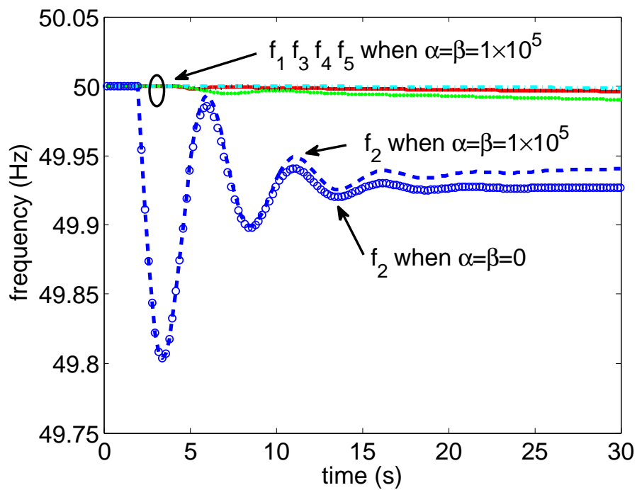
Figure 5.8: Frequencies of the five AC areas under the power-injection-based control scheme when \tau = 2\text{s} and \alpha = \beta = 1 \times 10^5 . The evolution of f_2 when \alpha = \beta = 0 is also shown.
