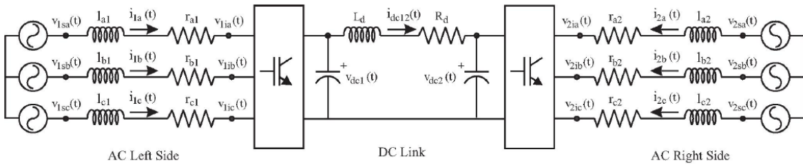
Figure 3.8: Three-phase diagram of a VSC-base HVDC link.
