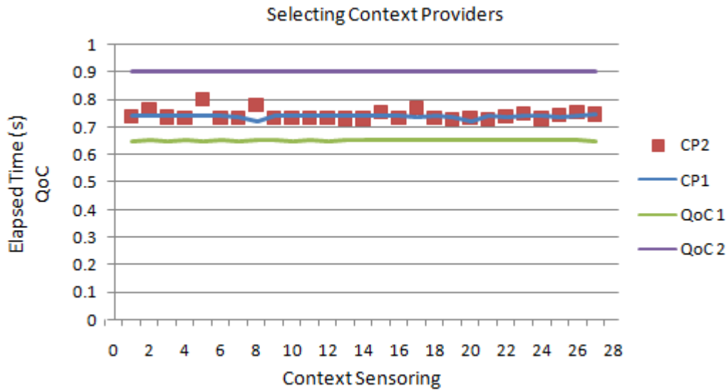
Figure 7.10: QoC-based and FIFO-based selection approaches.
