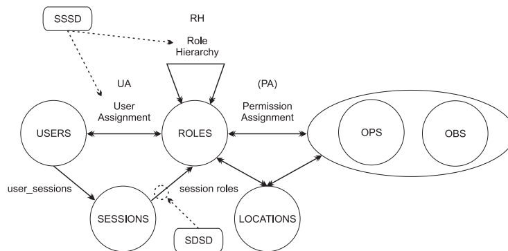
Figure 2.19: Spatial Role-Based Access Control Model (SRBAC) [Hansen 2003].
