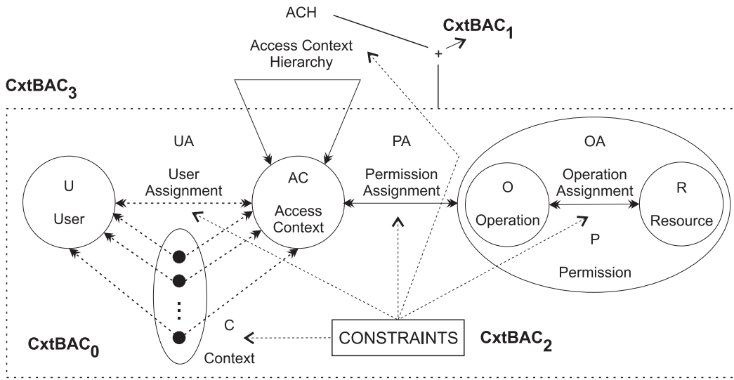
Figure 6.7: CxtBAC 3 - The core model.
