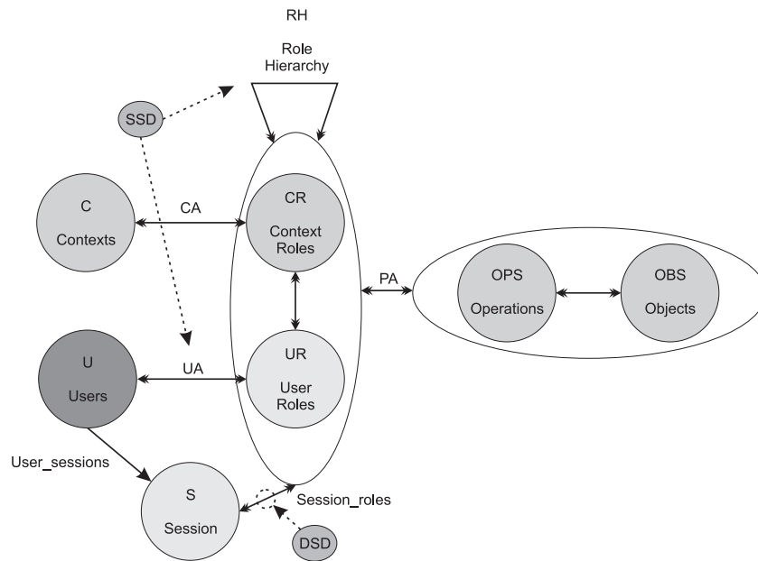
Figure 3.9: Context-Role Based Access Control Model (CRBAC) [Park 2006].
