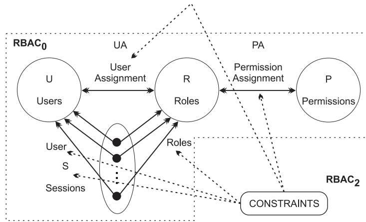
Figure 2.11: RBAC 2 : Constraints [Sandhu 1996].
