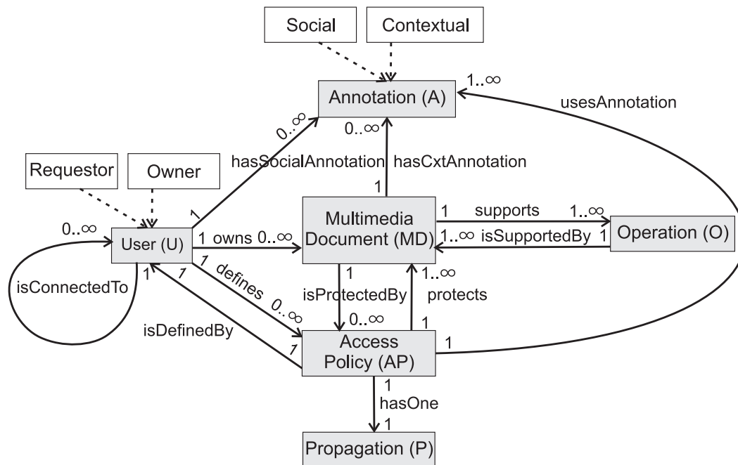
Figure 8.2: CxtANBAC - Contextual Annotation-based access control.
