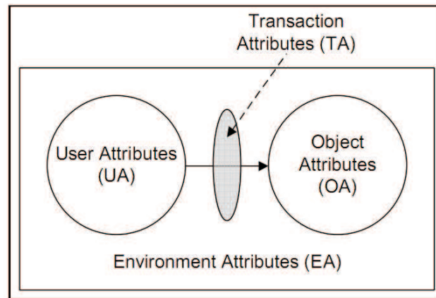
Figure 3.13: Transaction Overview using Contextual Attributes [Covington 2006].
