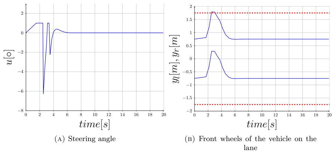
FIGURE 10.6: Simulation for the straight road segment.
