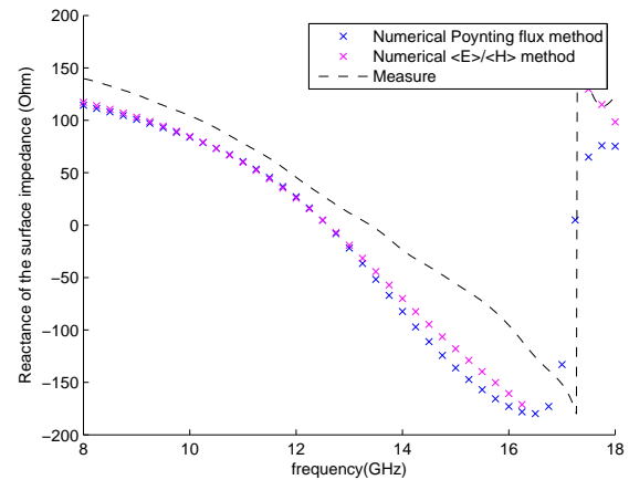
Figure 4.17: Numerical and experimental results for Sample J2
