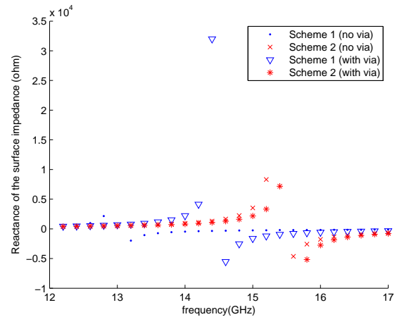
Figure 3.9: The influence of the via for the Jerusalem structure
