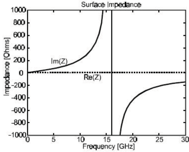
Figure 1.12: An example of the surface impedance curve for a mushroom HIS structure
