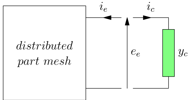
Figure 5.2: A lumped element is connected to an edge element
