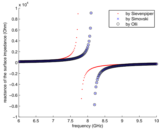
Figure 2.18: Comparison of surface impedances as calculated by different analytical methods for a Mushroom structure ( D = 2.4 mm, g = 0.015 mm, h = 1.6 mm, \epsilon_r = 4.4 )
