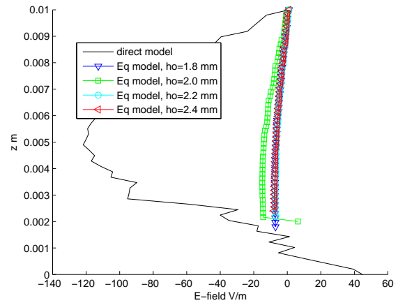
Figure 5.19: E-field in different models at 12 GHz. (The equivalent models are based on the surface impedance obtained by the \langle E \rangle / \langle H \rangle method.)
