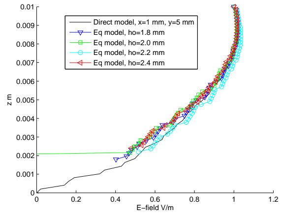
Figure 5.11: Study on different observation surface heights with the \langle E \rangle / \langle H \rangle method, at 8 GHz, Line 2
