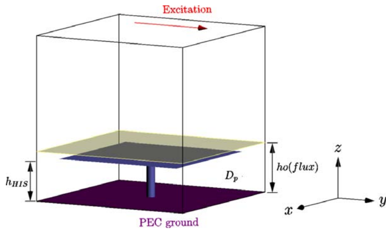
Figure 3.26: Illustration of the study domain for the Poynting flux method
