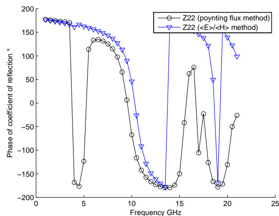
Figure 3.53: Reflection phase of four spiral-arm HIS structure
