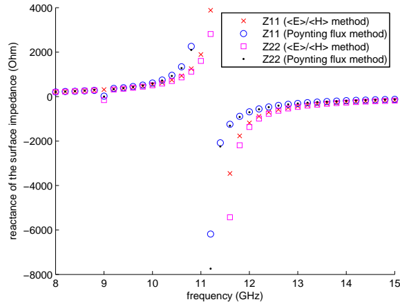
Figure 3.29: 2D calculations of Z_{11} and Z_{22} for a mushroom structure
