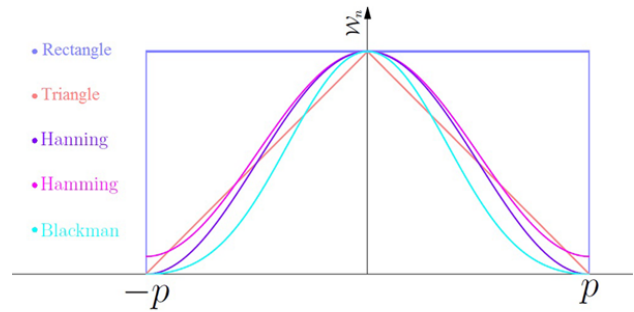
Figure 4.7: Filters with different windows
