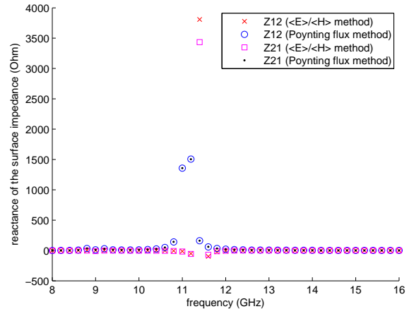
Figure 3.30: 2D calculations of Z_{12} and Z_{21} for a mushroom structure
