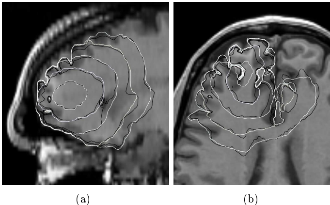
Figure 4.6: The temporal evolution of the iso-density contour is demonstrated for a synthetic tumor. Contours are shown for days 400, 600, 800, 1000 and 1200 from the innermost to outermost respectively. The synthetic tumor is virtually grown using the reaction-diffusion model. White contours are obtained by thresholding the tumor cell densities at u = 0.4 for the respective day values (400-600-800-1000-1200). Then in order to simulate the evolution of the iso-density contour (assumed to correspond to tumor delineation in real images) starting from day=400, without the knowledge of the tumor cell density distribution we use the traveling time formulation. Black curves are the contours we obtain at days 600 (2nd innermost) to 1200 (outermost). We notice that the traveling time formulation is quite accurate in describing the evolution of the tumor delineation in the case of synthetic tumors. The tumors were grown in the images of a healthy subject for whom we also have the DT-MRIs. Parameters: ( d_w = 0.25 \text{ mm}^2/\text{day}, d_g = 0.01 \text{ mm}^2/\text{day}, \rho = 0.012 \text{ day}^{-1} T_0 = 400 \text{ days} ) The number of iterations for including the curvature effect in this example was 4.
