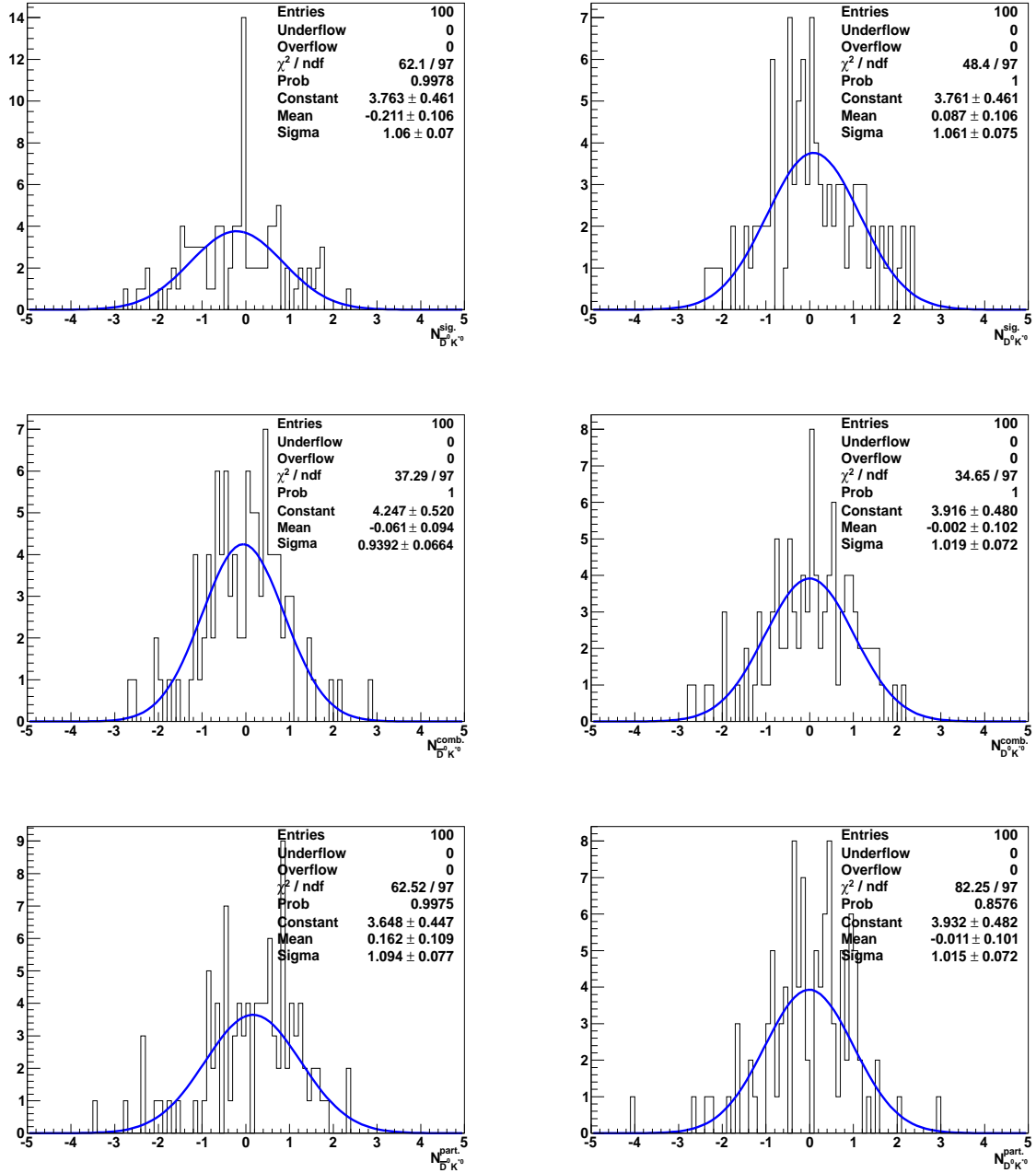
Figure A.2: Pulls of the yields (signal on the top, combinatorial background on the middle and partially reconstructed on the bottom) of the D0Kstar0 categories (D0Kstar SameSign on the left, D0Kstar OppositeSign on the right) in the fitting range (with c_{D^0K^{*0}}^{\text{part.}} fixed).
