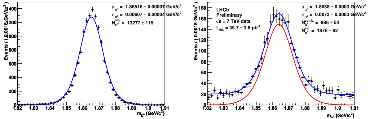
Figure V.20: D^0 mass distributions on Monte Carlo and real data respectively on the left and the right hand sides of the figure, in the \bar{B}_s^0 \rho^0 selection. All the selection cuts have been applied except the D^0 and B^0 mass requirements. The fit consists of a single Gaussian to model the signal shape plus a first order polynomial background in the real data.
