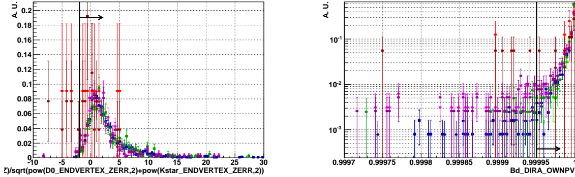
Figure IV.33: Distributions of the signed significance of the distance between the D^0 and K^{*0} positions of the vertex projected on the z -axis (left) and pointing angle of the B^0 (right). The final selection cut is materialized by the vertical bar and the arrow showing the events kept after the cut. In each plot, the red points corresponds to b\bar{b} -inclusive background, the blue points correspond to the properly reconstructed (and matched) B^0 \rightarrow \bar{D}^0 K^{*0} events, the green points correspond to partially reconstructed signal for which one of the two photons used to construct the \pi^0 is from the underlying event and the pink points correspond to the combinatorial background in the signal Monte Carlo data sample. The light and dark points respectively correspond to the events without and with a constraint on the D^0 invariant mass.
