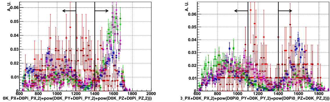
Figure IV.31: Distributions of the K^\pm\pi^\mp (left) and K^\pm\pi^0 (right) invariant masses. The final selection cut is materialized by the vertical bar and the arrow showing the events kept after the cut. In each plot, the red points corresponds to b\bar{b} -inclusive background, the blue points correspond to the properly reconstructed (and matched) B^0 \rightarrow \bar{D}^0 K^{*0} events, the green points correspond to partially reconstructed signal for which one of the two photons used to construct the \pi^0 is from the underlying event and the pink points correspond to the combinatorial background in the signal Monte Carlo data sample. The light and dark points respectively correspond to the events without and with a constraint on the D^0 invariant mass.
