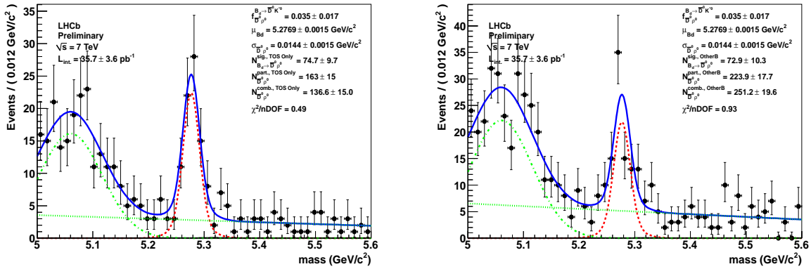
Figure V.45: Result of the fit for the B^0 \rightarrow \bar{D}^0 \rho^0 categories. The signal is clearly visible on the two figures corresponding to the two trigger categories (L0HadronTOSOnly on the left and OtherB on the right). The black points correspond to the data and the fit result is represented as a solid blue line. The signal is fitted with a double Gaussian (dashed red line), the partially reconstructed with a wide Gaussian function (green dash-dotted line) and the combinatorial background with a linear distribution (dashed green line) as explained in the text. Contributions from cross-feed are plotted in thin solid black lines.
