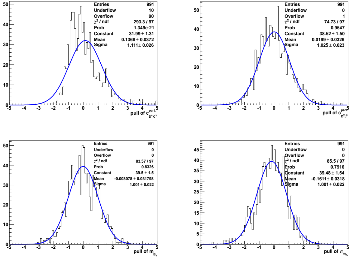
Figure V.29: Pulls of the shape parameters. The slope of the partially reconstructed background in D0Kstar0 (left) and D0rho0 (right) is shown on the top of the figure. Signal B^0 \rightarrow \bar{D}^0 \rho^0 mass (left) and resolution (right) is shown on the bottom plots.
