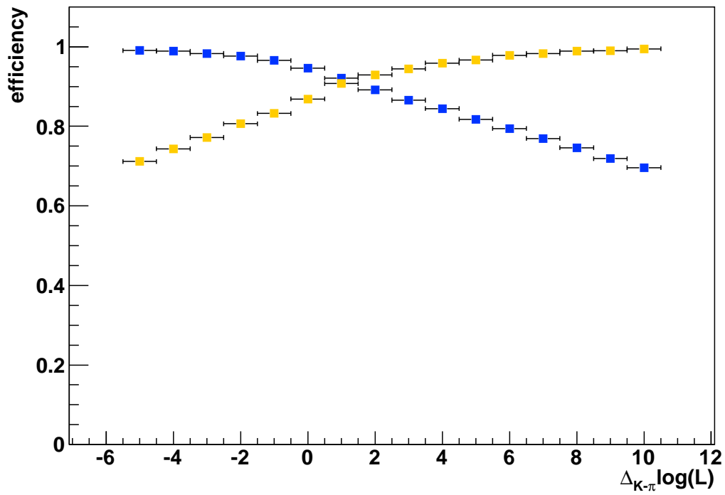
Figure V.15: Variation of the particle identification efficiency as a function of the threshold on \Delta_{K-\pi} \log L . This has been produced from the full data sample of D^0 candidates. The blue (dark grey in black and white printing) curve corresponds to the kaon efficiency and the orange (light grey in black and white printing) curve to the pion efficiency.
