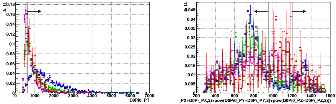
Figure IV.30: Distributions of p_T of the \pi^0 (left) and invariant \pi^\pm\pi^0 mass (right). The final selection cut is materialized by the vertical bar and the arrow showing the events kept after the cut. In each plot, the red points corresponds to b\bar{b} -inclusive background, the blue points correspond to the properly reconstructed (and matched) B^0 \rightarrow \bar{D}^0 K^{*0} events, the green points correspond to partially reconstructed signal for which one of the two photons used to construct the \pi^0 is from the underlying event and the pink points correspond to the combinatorial background in the signal Monte Carlo data sample. The light and dark points respectively correspond to the events without and with a constraint on the D^0 invariant mass.
