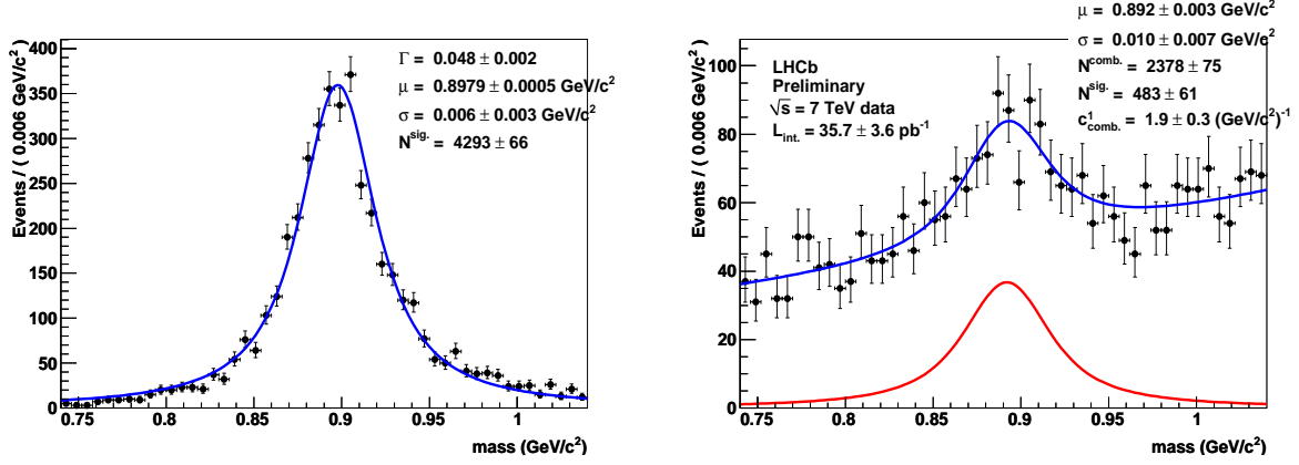
Figure V.21: K^{*0} mass distributions on Monte Carlo and real data respectively on the left and the right hand sides of the figure. All the selection cuts have been applied except the K^{*0} and B^0 mass requirements. The Monte Carlo corresponds to the B^0 \rightarrow D^0 K^{*0} signal only. The \bar{B}_s^0 \rightarrow D^0 K^{*0} fit result is in very good agreement and not shown here. The fit consists of a single Voigtian function given in Eq. V.4 (of which the intrinsic width is fixed to the PDG value) to model the signal shape plus an exponential background in the real data.
