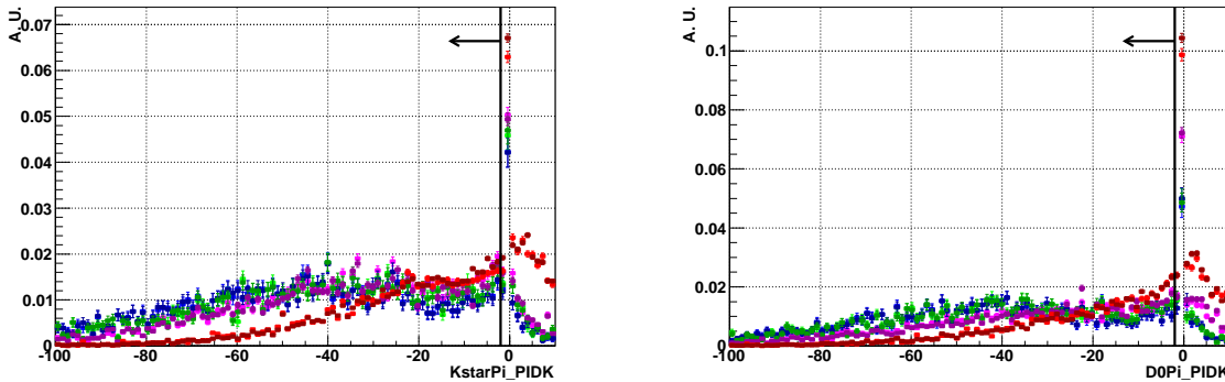
Figure IV.25: Distribution of the \text{DLL}_{K\pi} variable for the pions coming from the K^{*0} (left) and D^0 (right). The final selection cut is materialized by the vertical bar and the arrow showing the events kept after the cut. In each plot, the red points corresponds to b\bar{b} -inclusive background, the blue points correspond to the properly reconstructed (and matched) B^0 \rightarrow \bar{D}^0 K^{*0} events, the green points correspond to partially reconstructed signal for which one of the two photons used to construct the \pi^0 is from the underlying event and the pink points correspond to the combinatorial background in the signal Monte Carlo data sample. The light and dark points respectively correspond to the events without and with a constraint on the D^0 invariant mass.
