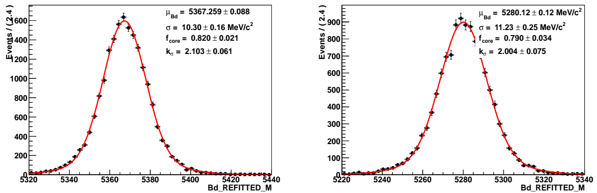
Figure V.24: Mass distribution in the \bar{B}_s^0 \rightarrow D^0 K^{*0} (left hand side of the figure) Monte Carlo 2010 simulation constraining the D^0 mass to its PDG value. The distribution is fitted with a double Gaussian. On the right hand side of the figure, the mass distribution for the \bar{B}^0 \rightarrow D^0 \rho^0 Monte Carlo 2010 simulation constraining the D^0 mass to its PDG value is shown. The core Gaussian resolution is higher by 9 \pm 3\% while the other fit parameters are fully consistent.
