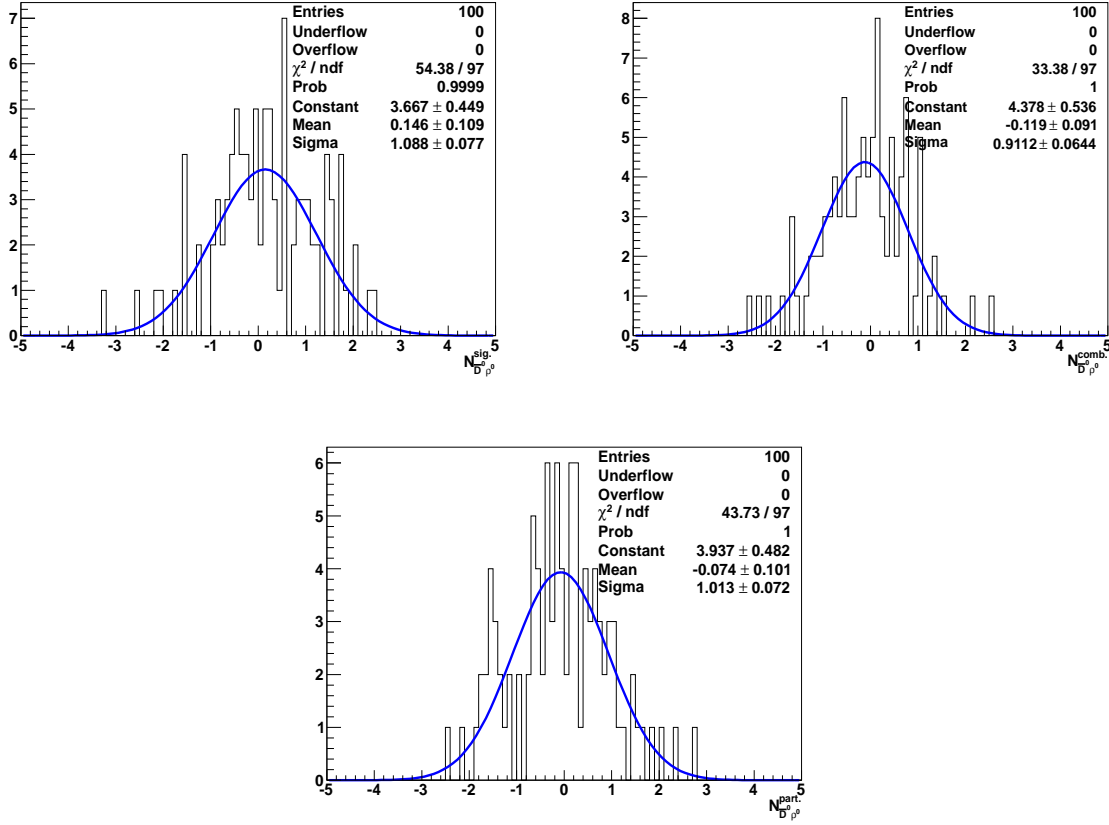
Figure A.1: Pulls of the yields (signal on the top left, combinatorial background on the top right and partially reconstructed background on the bottom) of D0 \rho^0 categories in the fitting range (with c_{D^0K^*0}^{\text{part.}} fixed).
