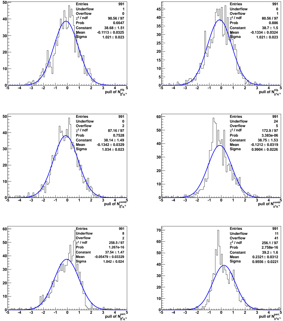
Figure V.28: Pulls of the yields (signal on the top, combinatorial background on the middle and partially reconstructed on the bottom) of the D^0 K^{*0} categories ( D^0 K^{*0} SameSign on the left, D^0 K^{*0} OppositeSign on the right) in the fitting range.
