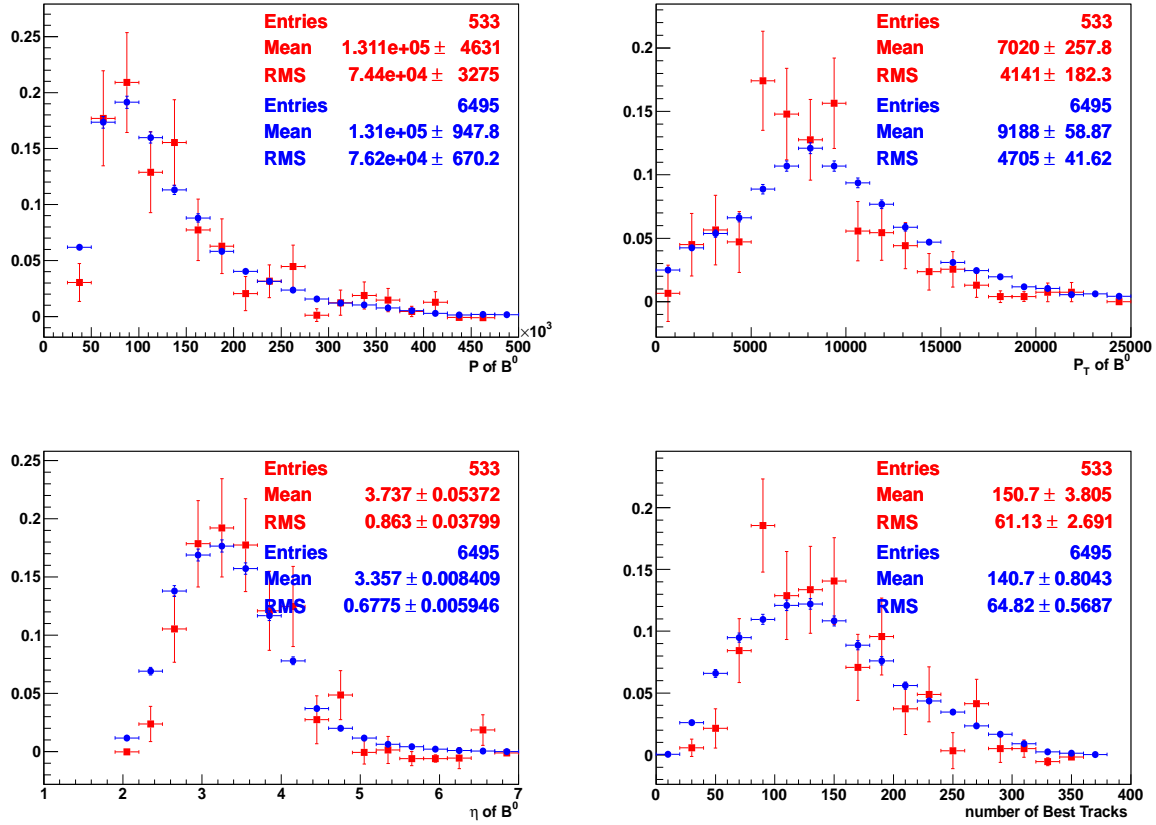
Figure V.34: sPlots in the D^0\rho^0 category (red points) and Monte Carlo prediction superimposed (blue points). The momentum and the transverse momentum of the B^0 are respectively given in the top left and right plots. The \eta distribution and the number of best tracks are given in the bottom distributions on the left and right of the figure respectively. While there is in general a good agreement between data and Monte Carlo, the momentum spectra seem a bit harder in the real data plots. The number of tracks is slightly underestimated in the Monte Carlo.
