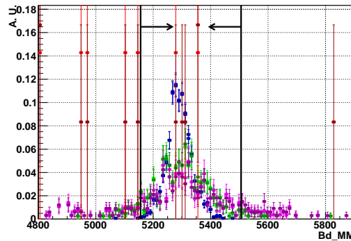
Figure IV.34: Distributions of the B^0 invariant mass. The final selection cut is materialized by the vertical bar and the arrow showing the events kept after the cut. In each plot, the red points corresponds to b\bar{b} -inclusive background, the blue points correspond to the properly reconstructed (and matched) B^0 \rightarrow \bar{D}^0 K^{*0} events, the green points correspond to partially reconstructed signal for which one of the two photons used to construct the \pi^0 is from the underlying event and the pink points correspond to the combinatorial background in the signal Monte Carlo data sample. The light and dark points respectively correspond to the events without and with a constraint on the D^0 invariant mass.
