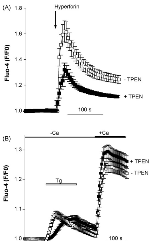
Fig. 4. (A and B) The Zn 2+ chelator TPEN diminishes the hyperforin-sensitive responses without altering the Tg-dependent Ca 2+ entry. In this set of experiments, the Zn 2+ chelator TPEN (10 \mu M) was added 1–2 min before the beginning of the recording and remained present in the bath. It partially reduces the amplitude of the peak and the plateau phase observed in response to the addition of hyperforin (10 \mu M) whereas it failed to block the Tg-dependent Ca 2+ responses. The total number of cells and dishes used was: 54/3 (hyperforin), 67/3 (hyperforin + TPEN), 85/3 (Tg), and 86/3 (Tg + TPEN).
