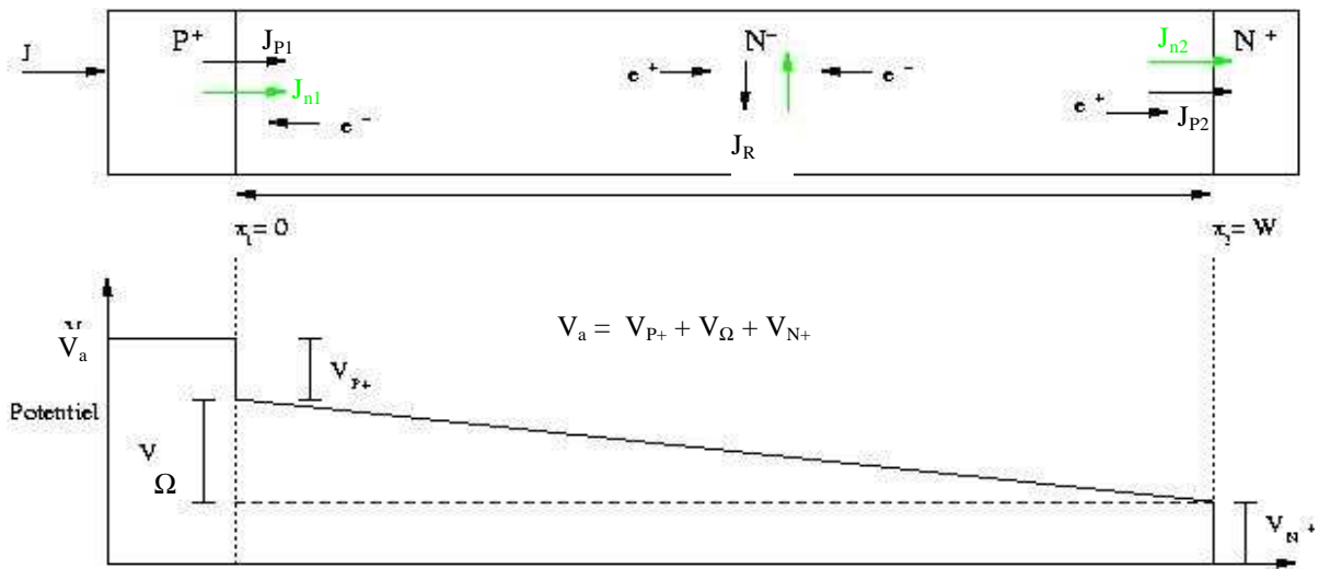
Figure 2. Diode PIN
