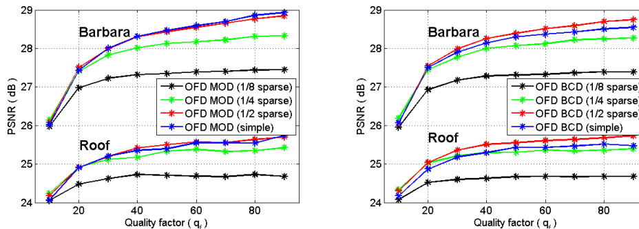
Figure 4.6: Prediction performance curves of Barbara and Roof using on-the-fly dictionaries: (left) MOD and (right) BCD with various sparsity constraints - PSNR performance curves with different quality levels in the image coding scheme. Optimization criterion is the minimization of the prediction signal SSE.
