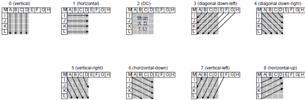
Figure 2.10: Nine prediction modes of H.264/AVC Intra-4 × 4 type - Unknown pixels are predicted using pixels A-M. The prediction is done by simply propagating (or interpolating) the pixel values along the specified direction.
