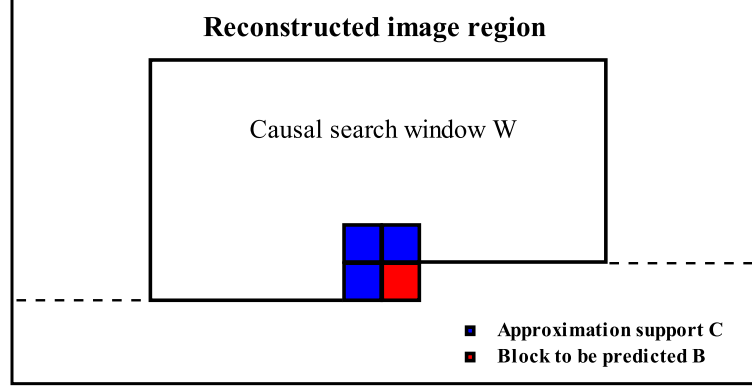
Figure 4.1: Online prediction dictionary learning - C is the approximation support of the current n \times n block to be predicted B. W is the search window from which texture patches are extracted to collect the training samples for learning the dictionary \mathbf{A} to be used for the prediction of B.
