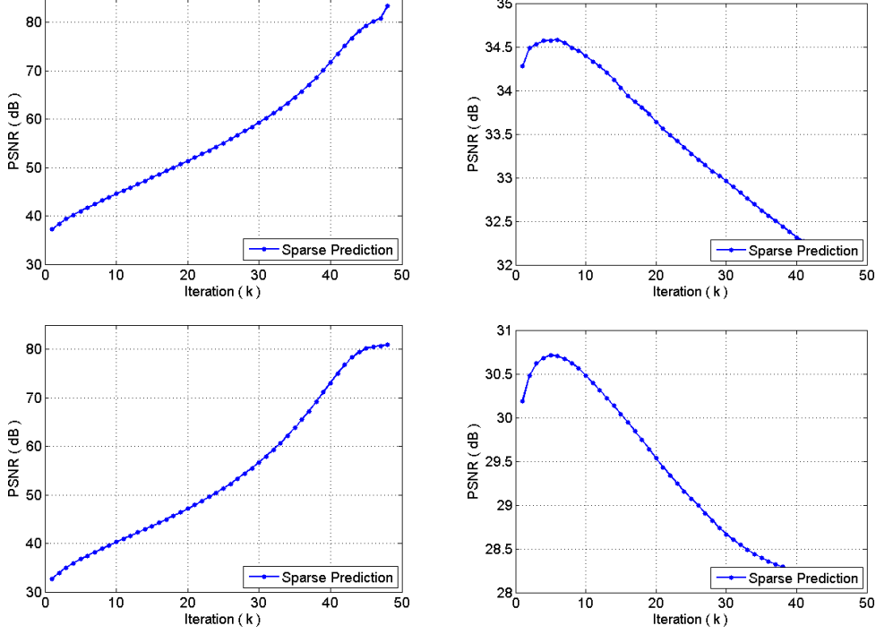
Figure 3.6: Mean prediction PSNR versus sparsity performance curves of (top) Foreman and (bottom) Barbara using sparse prediction - (left) The approximation support, (right) the unknown block. Block size is 4 \times 4 pixels, and the approximation support Mode 1 as illustrated in Fig. 3.5 has been used.
