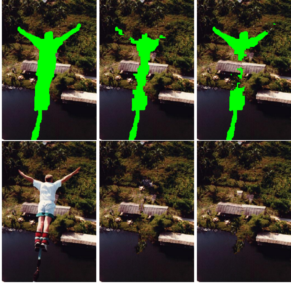
Figure 6.3: Effect of the edge term in the priority function - From top-to-bottom left-to-right: The mask for the inpainting algorithm and the original Bungee image; the inpainting process after 100 patches with priority function of [43] and the final inpainted image using TM; the inpainting process after 100 patches with the augmented priority function and the final inpainted image using TM.
