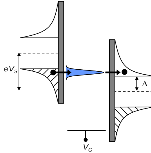
Figure 7.8: Adapted from [31]. Energy level diagram of a quantum dot in the weak coupling regime. Notice the width of the energy level in the dot which is much thinner than previously (strong coupling). The tunneling of Cooper pairs is suppressed. One needs to provide at least energy eV = 2\Delta for the quasiparticles tunneling to take place.
