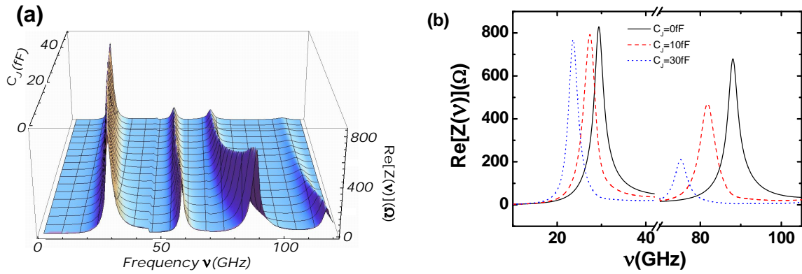
Figure 5.11: (a) 3D graph of Re[Z(\nu)] as a function of frequency and the junctions capacitance C_J (in parallel with resistor R_J = 10M\Omega ). The other parameters are fixed to R_{End} = 10M\Omega , R_{Loss} = 1.4M\Omega/m around \nu_1 , R_{Loss} = 5.5M\Omega/m around \nu_2 , R_{Loss} = 10M\Omega/m around \nu_3 .(b) Re[Z(\nu)] as a function of frequency for several junction capacitances C_J in the same conditions.
