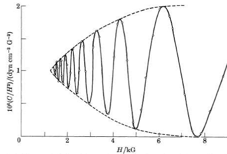
FIGURE 2. Oscillatory field dependence of torque for bismuth at T = 4.2 K. The ordinate is C/H^2 where C is the torque per unit volume at field H ; the field is at 9.7^\circ from the binary axis in the binary-trigonal plane. (Shoenberg 1939.)
