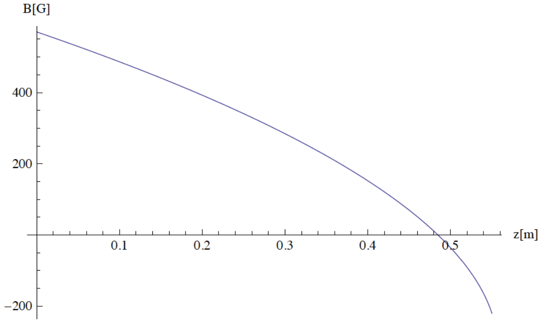
Figure 1.13: Ideal magnetic profile of the {}^6\text{Li} Zeeman slower, plotted from equation 1.8 with v_c = 838 \text{ m.s}^{-1} , l = 55 \text{ cm} , \delta = -75 \text{ } \Gamma and \alpha = 0.34 .
