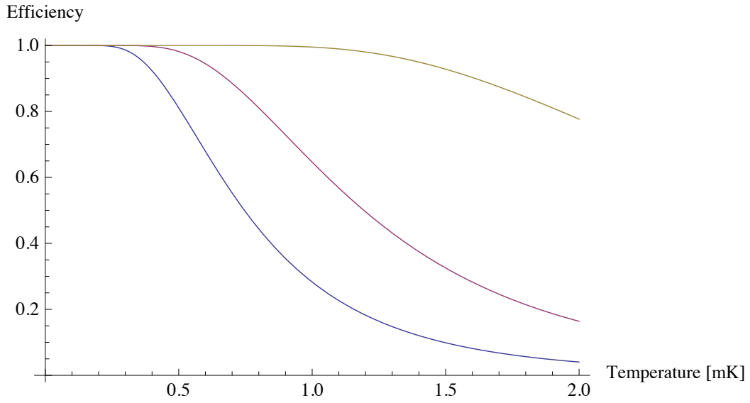
Figure 5.10: Theoretical efficiency of trapping {}^6\text{Li} and {}^{40}\text{K} atoms in a static magnetic trap of gradient 93\text{ G}\cdot\text{cm}^{-1} as a function of temperature, for three different tubes: DN10 (blue), DN16 (pink), and DN38 (yellow). The model used is given in equations 5.2 and 5.4.
