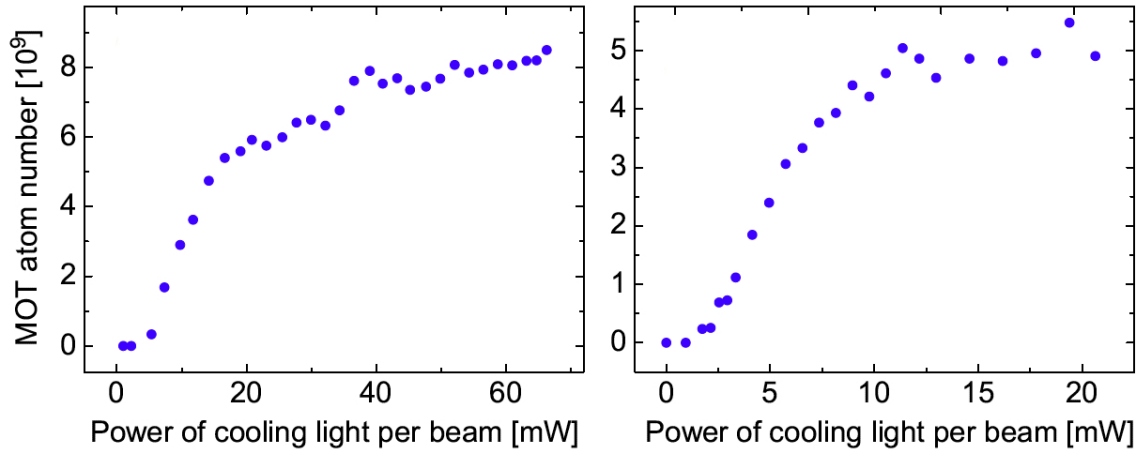
Figure 2.10: Number of atoms in each single-species MOT: ^{40}\text{K} (left) and ^6\text{Li} (right), as a function of the cooling power in each of the six beams.
