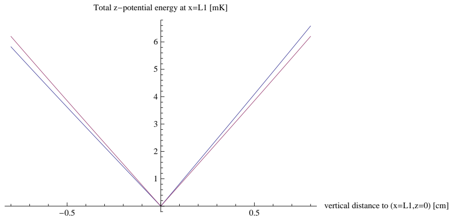
Figure 4.21: Vertical trap profile at x = L_1 , with (blue) and without (pink) the gravitational tilt. There the vacuum tube has a DN16 size (0.8 cm radius), and the position x = L_1 is 9 mm away from the DN10 transport tube (0.5 cm radius).
