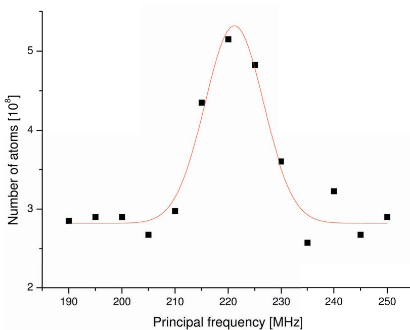
Figure 3.4: Dependency of ^{40}\text{K} atom number on the spin-polarization principal AOM frequency. The maximum corresponds to the atomic resonance. The picture has been taken after 54 ms in the magnetic trap and 2.1 ms of time-of-flight (see part 2.2.3).
