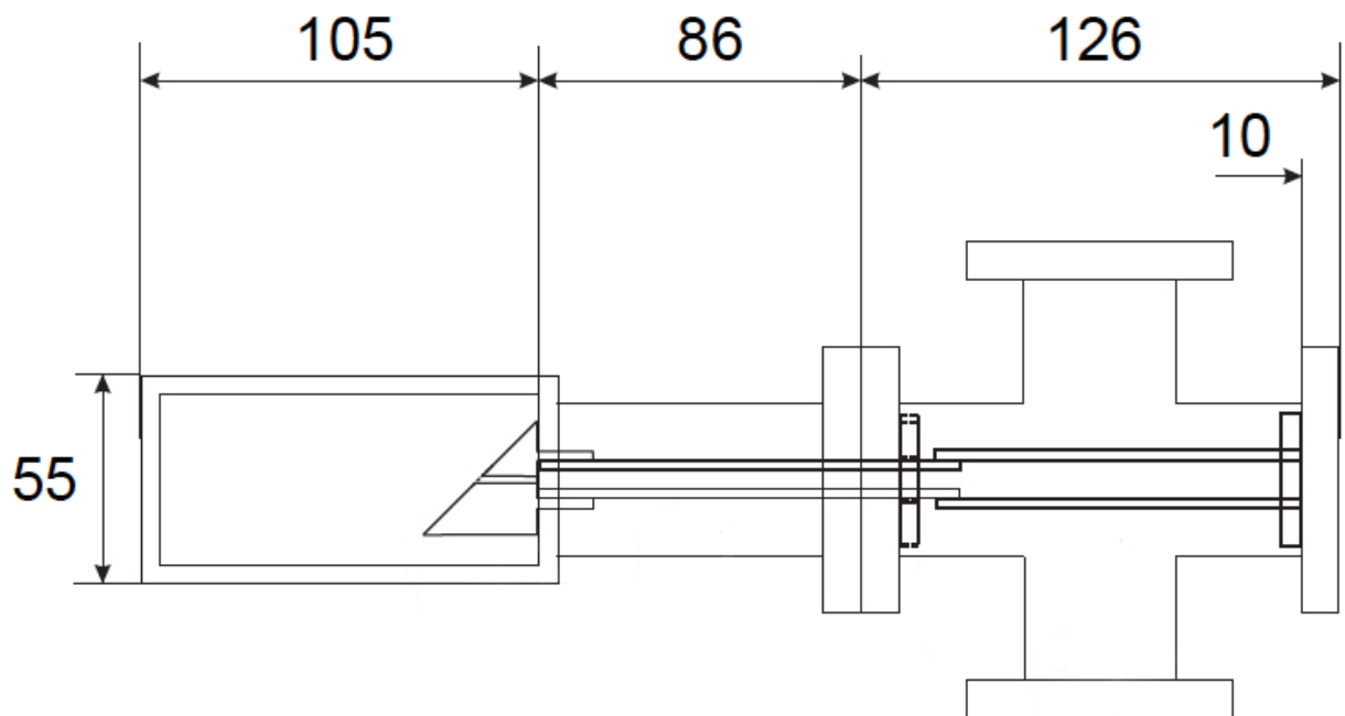
Figure A.4: 2D-MOT chamber with differential pumping tube inside (dimensions in millimeters). The differential pumping tube consists of three joined pipes: the cylinder hole in the mirror of 2 mm diameter and 20 mm length, a tube of 5 mm diameter and 116 mm length, and a tube of 10 mm diameter and 86 mm length.
