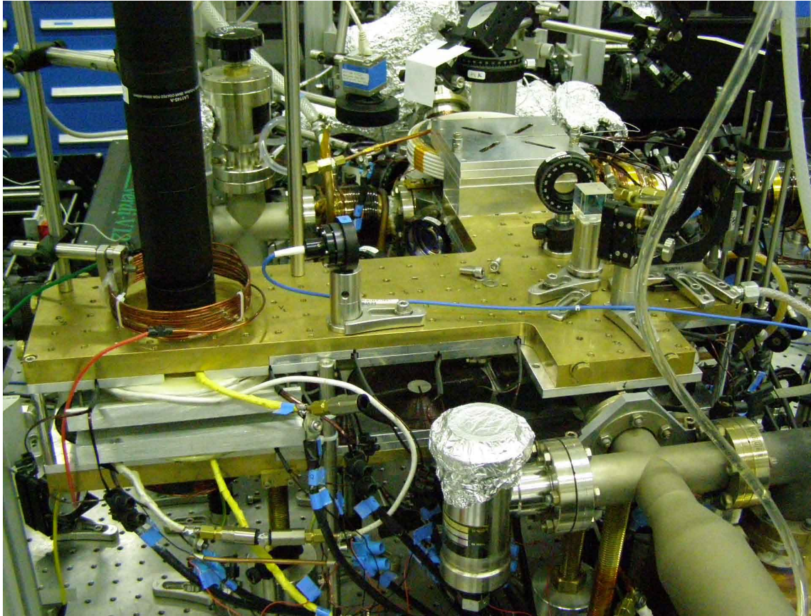
Figure 4.25: Full transport setup. See engineering drawings in appendix A.6.
