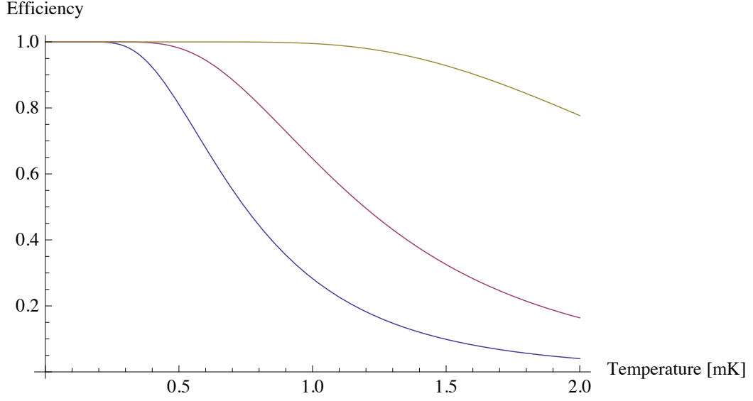
Figure 5.10: Theoretical efficiency of trapping ^6\text{Li} and ^{40}\text{K} atoms in a static magnetic trap of gradient 93 \text{ G.cm}^{-1} as a function of temperature, for three different tubes: DN10 (blue), DN16 (pink), and DN38 (yellow). The model used is given in equations 5.2 and 5.4.
