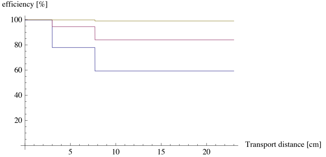
Figure 5.14: Theoretical transfer efficiency of {}^6\text{Li} and {}^{40}\text{K} as a function of transport distance, for three temperatures: 0.3 mK (yellow), 0.5 mK (pink), and 0.7 mK (blue). The model used is given in equations 5.2 and 5.4, and takes into account the full ramps on the gradients (see Figure 4.3).
