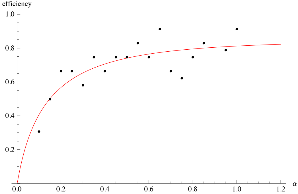
Figure 5.13: ^{40}\text{K} transfer efficiency at x = 9 \text{ cm} as a function of the gradient at x = 9 \text{ cm} . \alpha is the ratio between the y -gradient and the y -gradient of the normal sequence (see Figure 4.3). The initial number of atoms is 5 \times 10^8 and the initial temperature is 500 \mu\text{K} . The fit is based on equations 5.2 and 5.4, normalized by the vacuum losses in 1.6 \text{ s} . Its outputs are a radius of the tube of 6 \text{ mm} and an initial number of atoms of 4 \times 10^8 .
