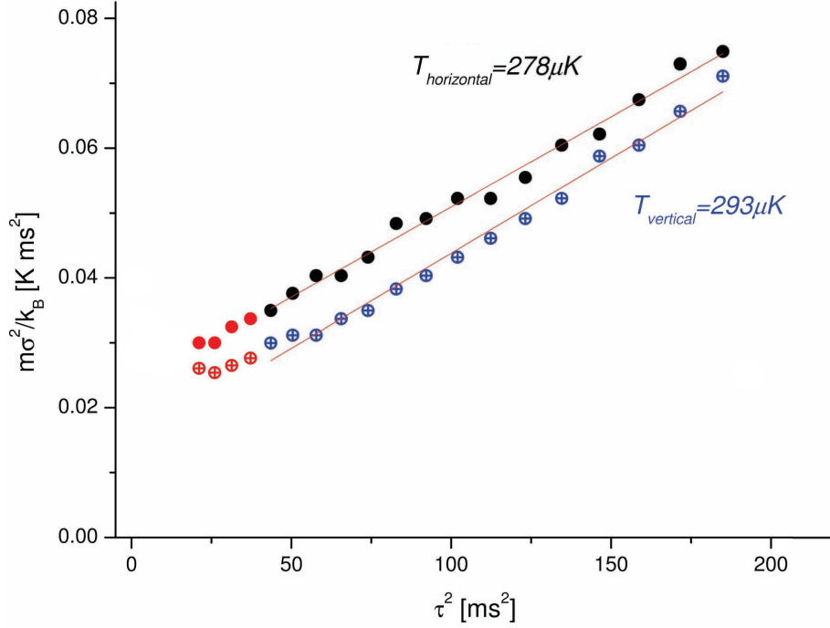
Figure 2.8: Time-of-flight measurement of ^{40}\text{K} MOT temperature (see equation 2.15).
