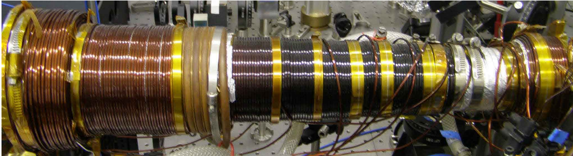
Figure 1.19: {}^6\text{Li} Zeeman slower.
