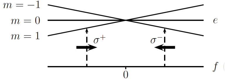
Figure 2.2: 1D principle of a magneto-optical trap. For a pedagogical purpose, we depicted a simple two level transition: from F = 0 to F' = 1 , in a quadrupolar field chosen to be positive on the right and negative on the left. Thus, the Zeeman effect increases the energy of m = 1 on the right, and decreases it on the left. Then, due to the positive helicity of both laser beams, we have a \sigma^- polarization on the right and a \sigma^+ one on the left. Since the beams are red-detuned, the beam coming from the right is more resonant with an atom placed on the right than the one coming from the left, leading to a pushing in the left direction, and thus a trapping at the center.
