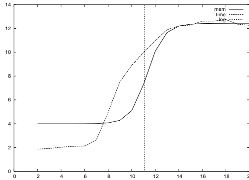
FIG. A.10 – Results obtained with the factor tree on the sequence with EMBL primary access number AE000111 . The Y-axis indicates the space occupied by the factor tree in bytes per input char and the execution time in seconds, the X-axis plots the values at which the tree is cut. The log curve represents \log_4 |s| .
