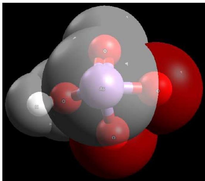
Figure 41: Hydrogen arsenate ( HAsO_4^{2-} ) with partial charge indicated by colour (white = neutral, red = negative). Constructed using Avogadro software.
