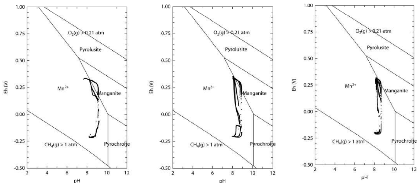
Figure 98: Pourbaix diagrams of the Mn – CO 2 – H 2 O system at 298.15K and 10 5 Pa. \Sigma Mn = 10^{-5} from LLNL data. Measured Eh pH conditions in reactor suspensions are overlaid in black (reactor 1 left, reactor 2 middle and reactor 3 right).
