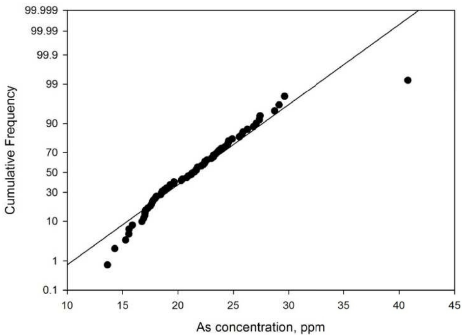
Figure 66: Arsenic concentration cumulative frequency plot. Normally distributed data would be expected to plot on a straight line whereas arsenic concentrations deviate significantly from this.
