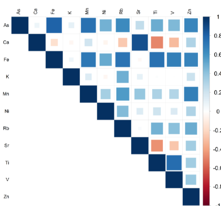
Summary Figure 5: Correlation matrix demonstrating inter-elemental relationships in soils on the Saône floodplain. Square size and colour corresponds to the correlation coefficient between elemental pairs (blue positively correlated, red negatively correlated).
