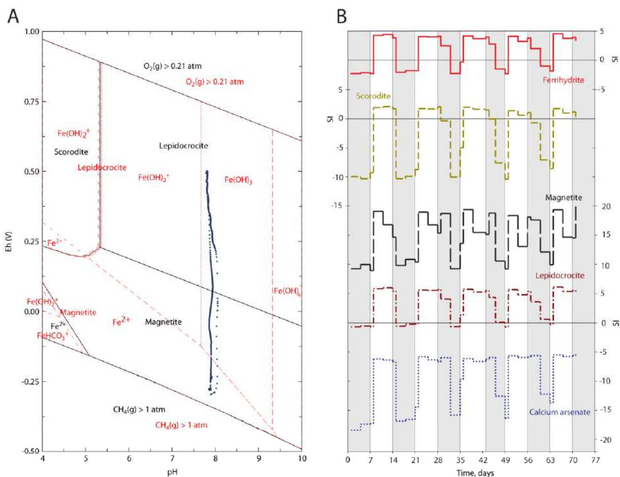
Figure 77: A: Pourbaix diagram of the Fe, As, CO 2 and H 2 O system in the reactor suspension with Fe as the principal species. Point data are measured Eh and pH couples from one full cycle. Dominant stability fields are shown with black solid lines and subdominant fields with red dashed lines. B: Saturation indexes of ferrihydrate (solid red line), scorodite (short dashed mustard line), magnetite (long dashed black line), lepidocrocite (dot/dashed line) and calcium arsenate (dotted line) with time during reactor experiments.
