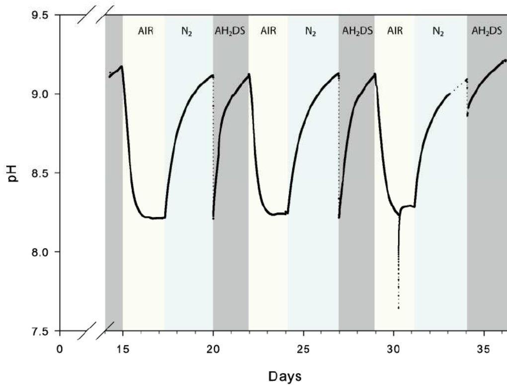
Figure 103: pH with time measured within the reactor 1 suspension, reference shading indicates; light yellow = initiation of air sparging, light blue = initiation of N_2 sparging, grey = addition of AH_2DS^{2-} reductant solution.
