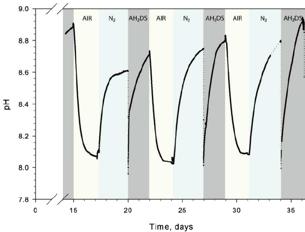
Figure 104: pH with time measured within the reactor 2 suspension, reference shading indicates; light yellow = initiation of air sparging, light blue = initiation of N_2 sparging, grey = addition of AH_2DS^{2-} reductant solution.
