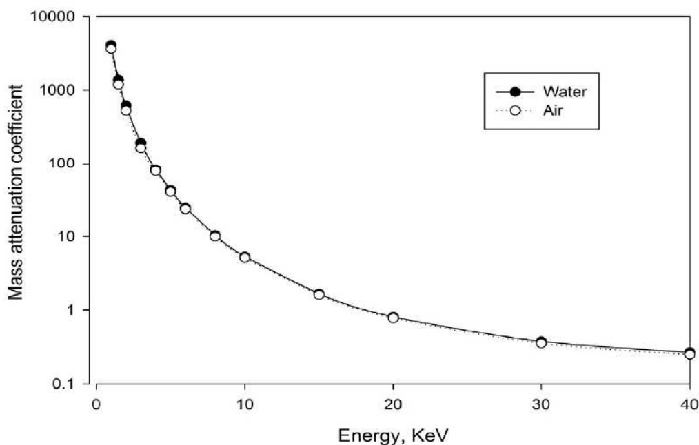
Figure 53: Mass attenuation coefficients for water and air across the energy range used in FP-XRF analysis. Data from Hubbell and Seltzer (2009)
