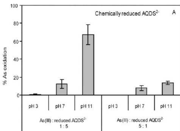
Figure 119: Oxidation of As(III) by chemically reduced AQDS 2- . The initial concentrations were 90 μM As(III) and 450 μM reduced AQDS 2- (molar ratio 1:5) or 330 μM As(III) and 67 μM reduced AQDS 2- (molar ratio 5:1). From Jiang et al. (2009).
