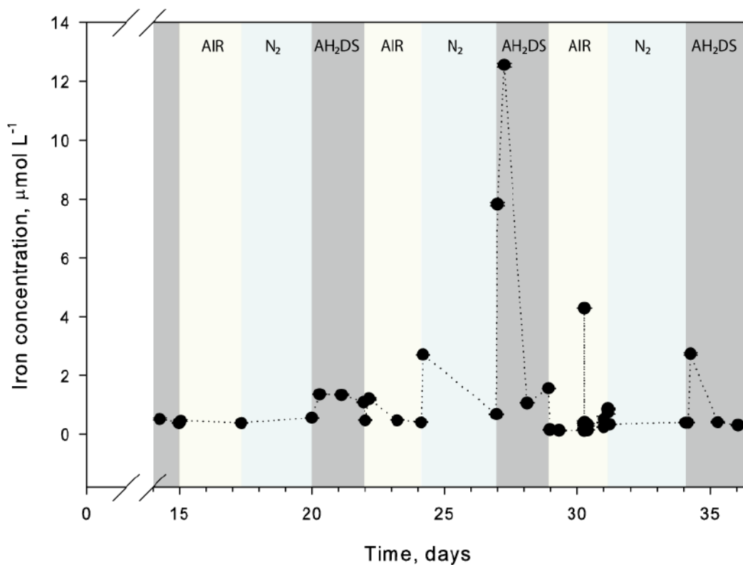
Figure 100: Aqueous/colloidal iron concentration in the reactor 1 suspension over time. The increases occurring on days 20, 27 and 34 are thought to be due to the release of \text{Fe}^{2+}_{(\text{aq})} following reduction by added \text{AH}_2\text{DS}^{2-} .
