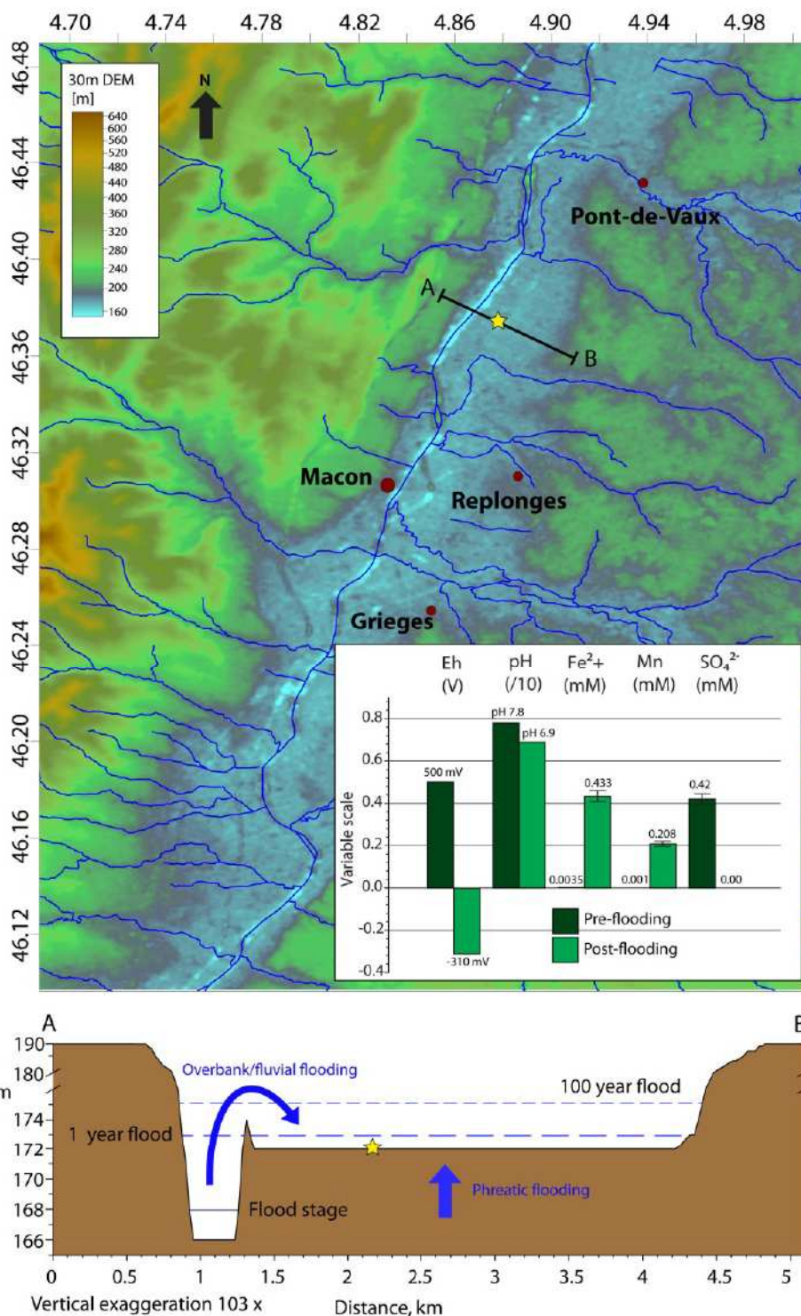
Figure 72: : TOP: Map of the extent of the Saône floodplain showing the sampling location (yellow star), towns (red circles), topography (METI/ERSDAC et al., 2009) and the hydrological network (Institut Geographique National de France, 2010)(in blue). Coordinates are in decimal degrees based on the WGS84 geoid. BOTTOM: An idealised cross-section of the floodplain at the sampling location illustrating the
