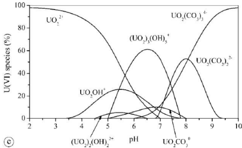
Figure 21: U(VI) speciation in 0.01M NaCl + 0.003M NaHCO 3 , [U] = 5 × 10 -5 M generated using PHREEQC and the WATEQ4F thermodynamic database (from Bachmaf et al. (2008)). . The formation of strongly anionic uranyl-carbonate-complexes at high pH is shown.
