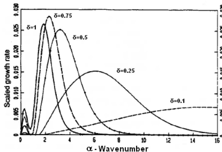
Figure 31: Dependence on wavenumber of the scaled growth rate with \beta = 0.2^\circ , \gamma = 0.4 and different depth ratios from [42].
