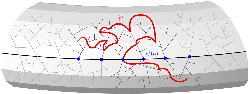
Figure 4.2. The set overflown by the path \wp is the set of (blue) large dots.
