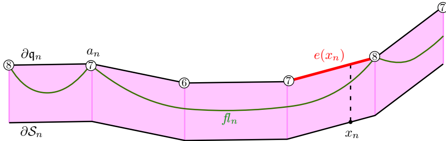
Figure 5.8. Approaching a point x_n \in \partial\mathcal{S}_n with a point a_n \in f\ell_n .
