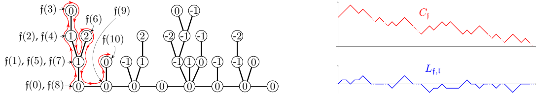
Figure 5.1. The facial sequence and contour pair of a well-labeled forest from \mathfrak{F}_7^{20} . The paths are dashed on the intervals corresponding to floor edges.
