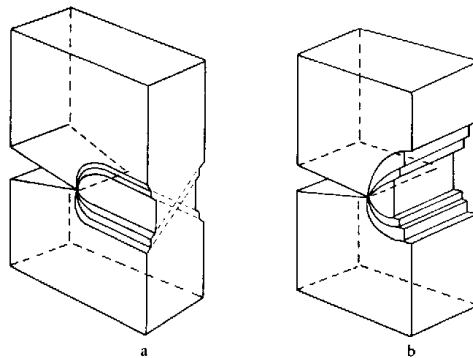
Figure 4.13. Deformation patterns a. 45° shear deformation in plane stress; b. Hinge type deformation in plane strain
