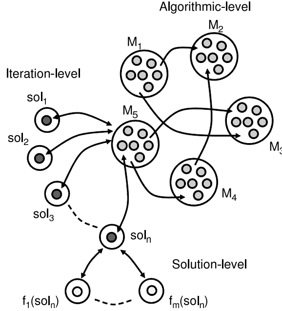
Figure 1.3: Parallel models of local search metaheuristics.
