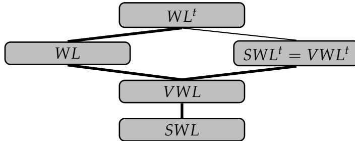
Figure 4.1: Expressive power of the rule languages (the inclusion is strict when the arc is in bold)
