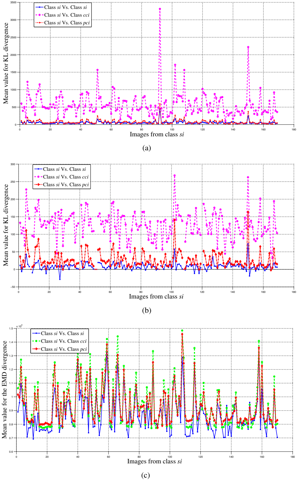
Figure 3.9: Mean values for the intra-class and inter-class divergence, (a) using the KL_{\text{simple}} divergence and (b) using the KL_{\text{app}} divergence and (c) using EMD on the histograms.
