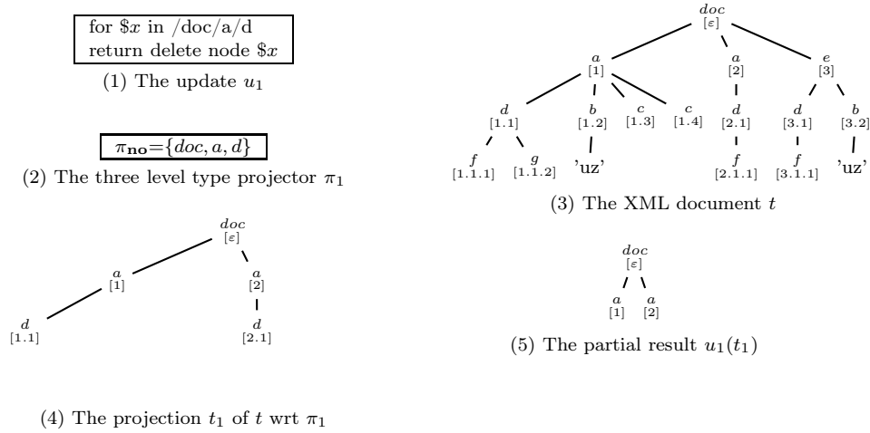
Figure 4.2: The projector component \pi_{no} , illustrated for "delete"
