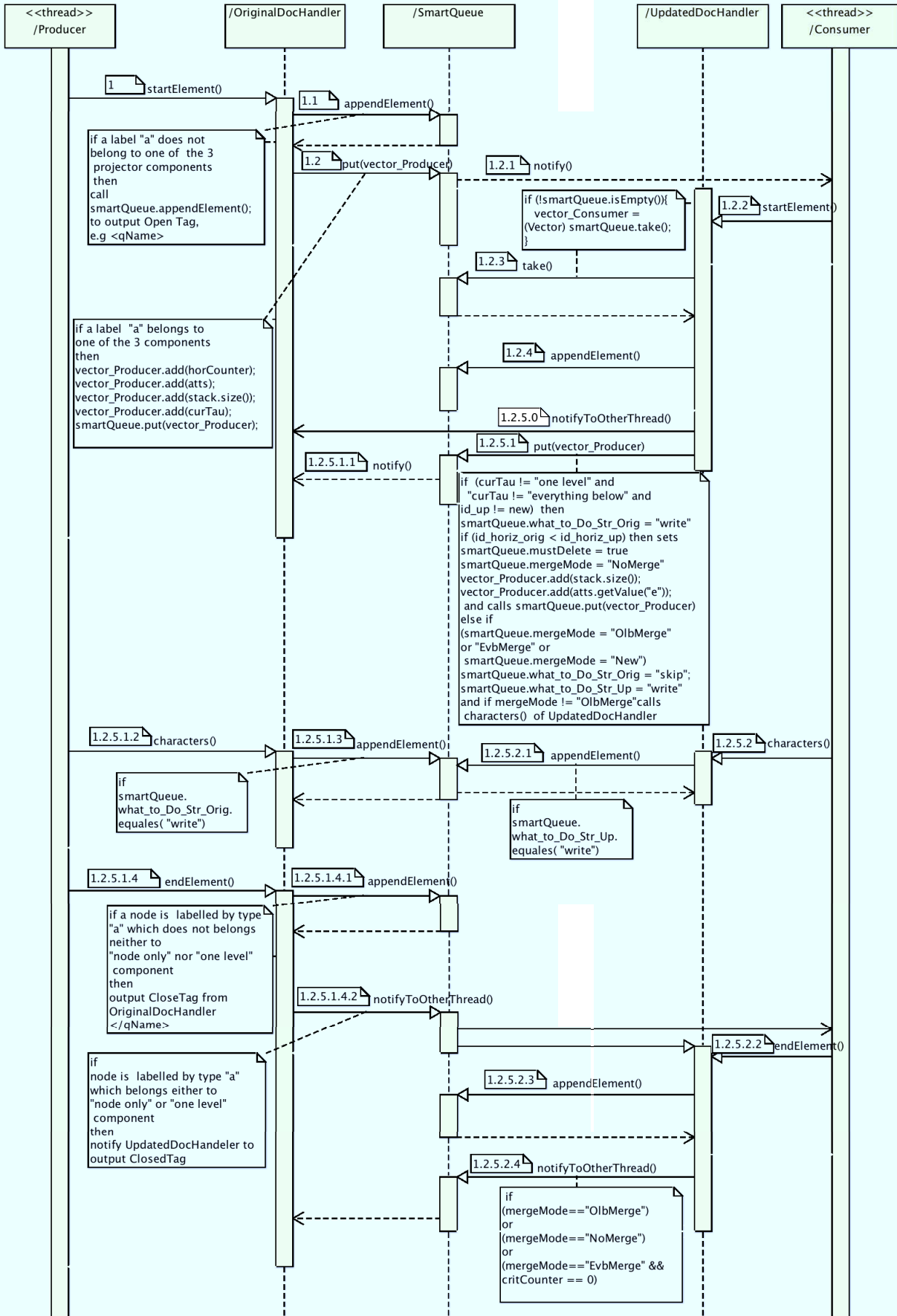
Figure 4.37: Sequence Diagram
