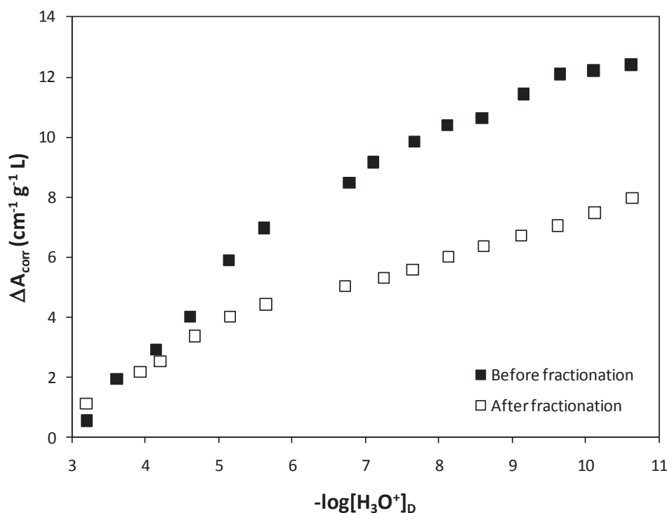
Figure 9. Spectrophotometric titration curve of PAHA before and after contact with \alpha\text{-Al}_2\text{O}_3 . I = 0.1 mol/L \text{NaClO}_4 .
