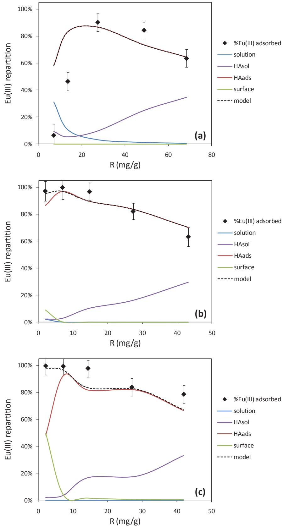
Figure 8. Eu(III) repartition in the ternary system depending on coverage ratio at (a) pH = 3.9 (b) pH = 6.2 ± 0.2 (c) pH = 7.4 ± 0.2. The dotted line "model" corresponds to the sum of "HAads" and "surface" lines.
