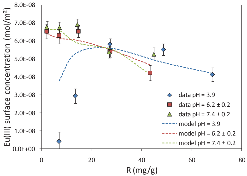
Figure 6. Eu(III) surface concentration in the ternary system depending on pH (a) and coverage ratio (b). Error bars correspond to 2\sigma .
