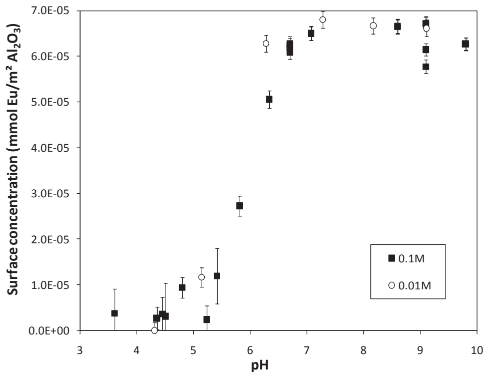
Figure 1. Surface concentration of Eu(III) onto \alpha -Al 2 O 3 depending on pH and I . [α-Al 2 O 3 ] = 1 g/L, [Eu(III)] = 10 -6 mol/L. Error bars correspond to 2σ.
