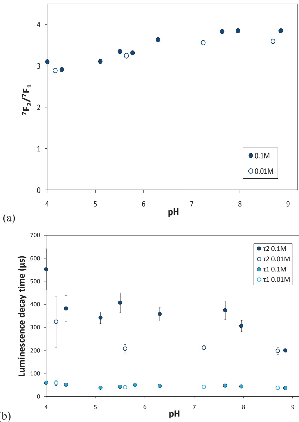
Figure 11. Asymmetry area ratios of Eu(III) luminescence spectra (a) and luminescence decay times of Eu(III) (b) in the ternary system at 0.01 and 0.1 M NaClO 4 depending on pH ( R = 27.4 \pm 0.5 \text{ mg}_{\text{PAHA}}/\text{g}_{\alpha\text{-Al}_2\text{O}_3} ).
