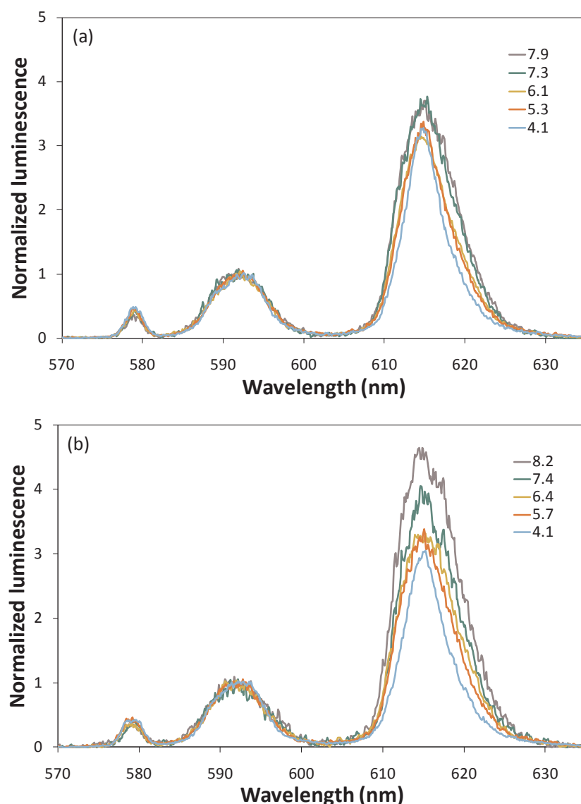
Figure 4. Eu(III) luminescence spectra at different pH in Eu(III)/PAHA system at 0.01 M (a) and 0.1 M (b) \text{NaClO}_4 . [\text{Eu(III)}] = 10^{-6} mol/L, [\text{PAHA}] = 25 mg/L.
