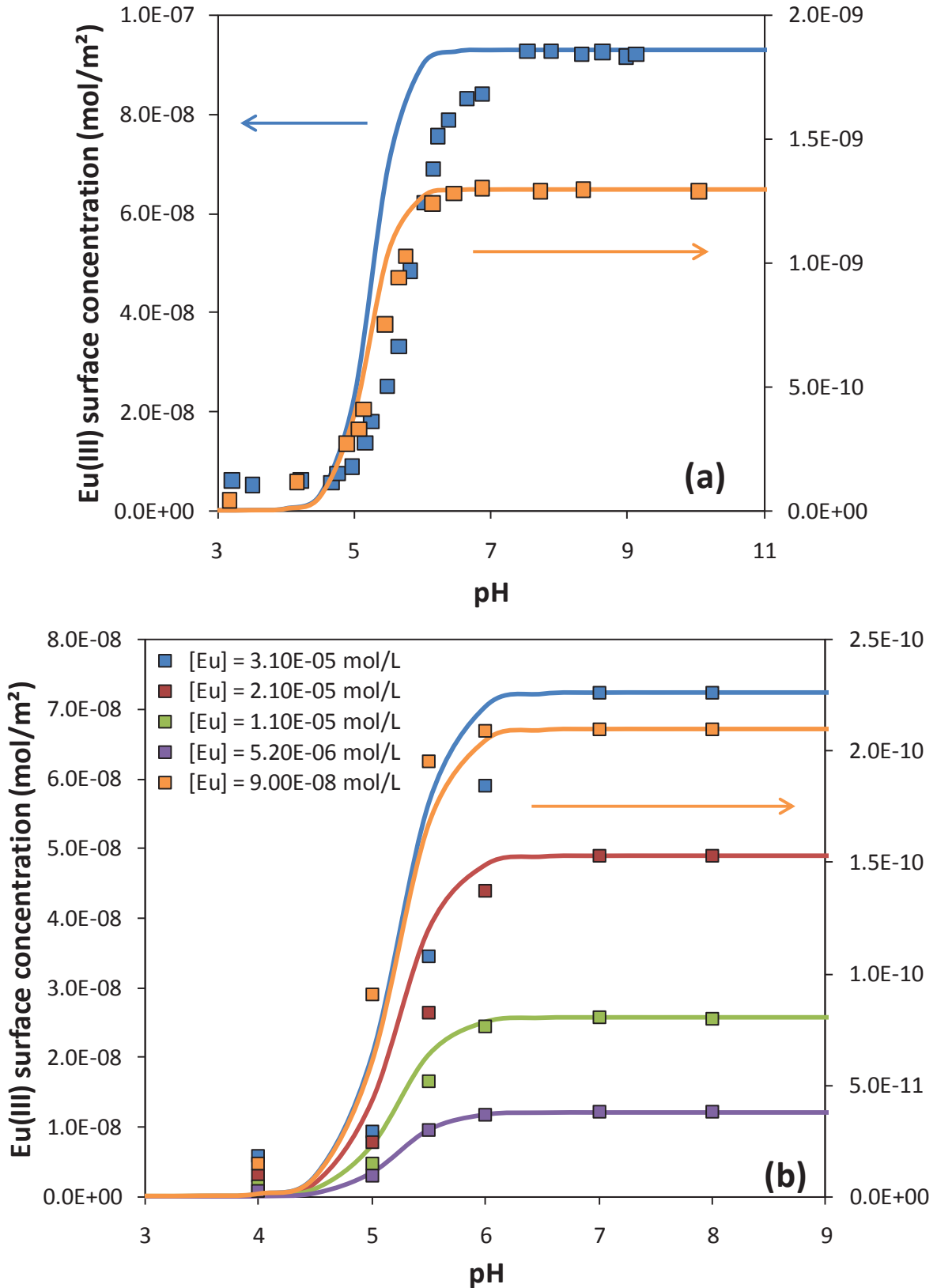
Figure 3. Eu(III) surface concentration on (a) 4.4 g/L hydrous alumina (105 m 2 /g), for I = 0.1 M KNO 3 and [Eu(III)] = 4.3 × 10 -5 mol/L (blue) and 0.1 M NaClO 4 and [Eu(III)] = 6.0 × 10 -7 mol/L (orange) (Tan et al. 2008) ; (b) 3.6 g/L γ-Al 2 O 3 (119 m 2 /g) for I = 0.1 M NaClO 4 and various Eu(III) concentrations (Rabung et al. 2000). Symbols are the data from literature, and lines are the results of the modeling presented in this study.
