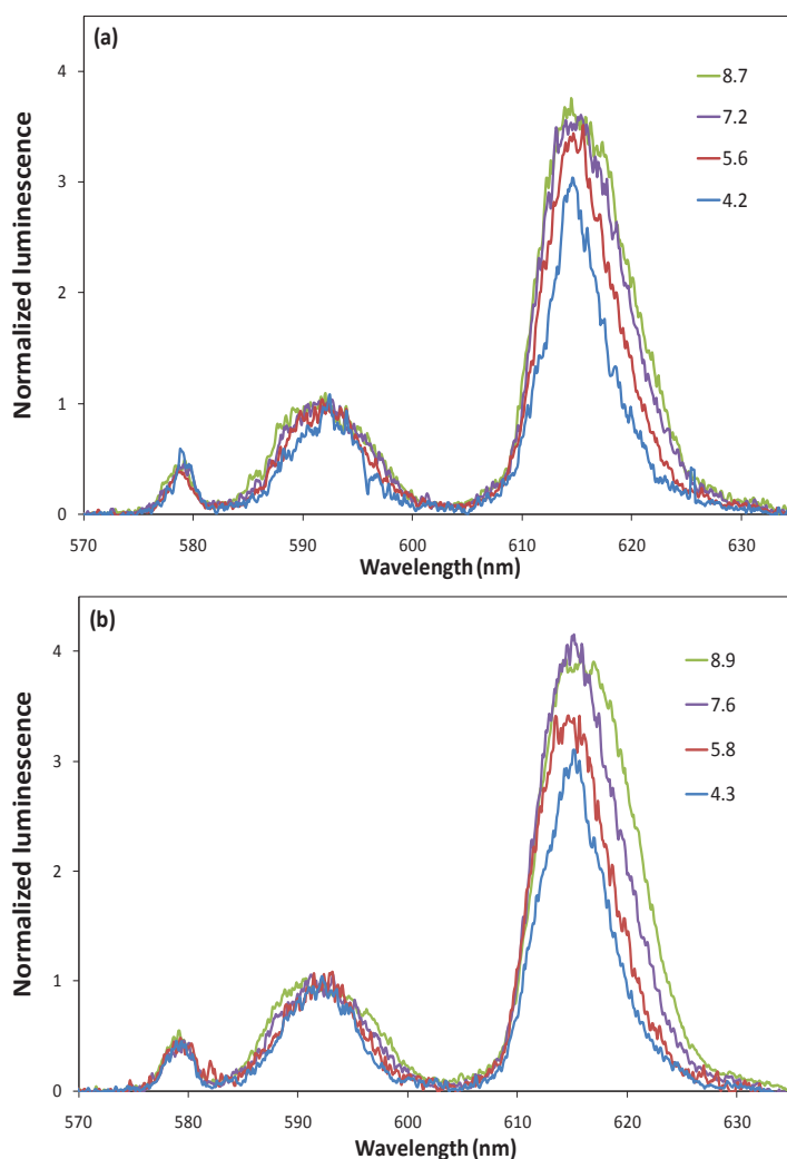
Figure 9. Eu(III) luminescence spectra in the ternary system at different pH at 0.01 M (a) and 0.1 M (b) NaClO 4 ( R = 27.4 \pm 0.5 \text{ mg}_{\text{PAHA}}/\text{g}_{\alpha\text{-Al}_2\text{O}_3} ).
