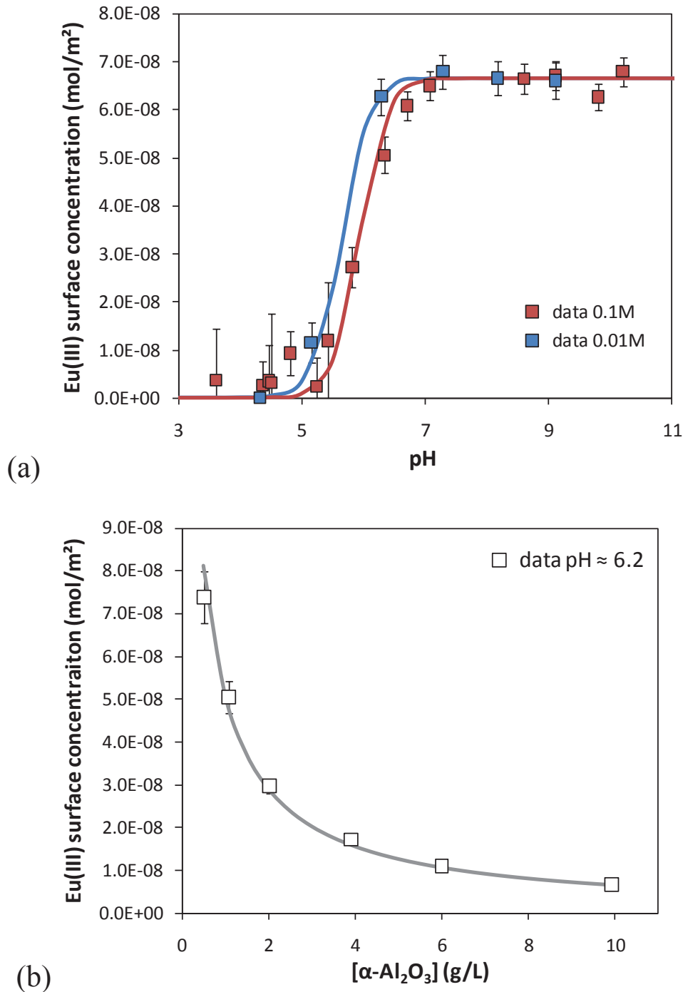
Figure 2. Surface concentration of Eu(III) in the binary Eu(III)/ \alpha -Al 2 O 3 system depending on pH (a) and \alpha -Al 2 O 3 concentration (b). The lines are the results of modeling. [Eu(III)] = 10 -6 mol/L; Error bars correspond to 2 \sigma . (a) [ \alpha -Al 2 O 3 ] = 1 g/L ; (b) I = 0.1 M NaClO 4 and pH = 6.2 \pm 0.1.
