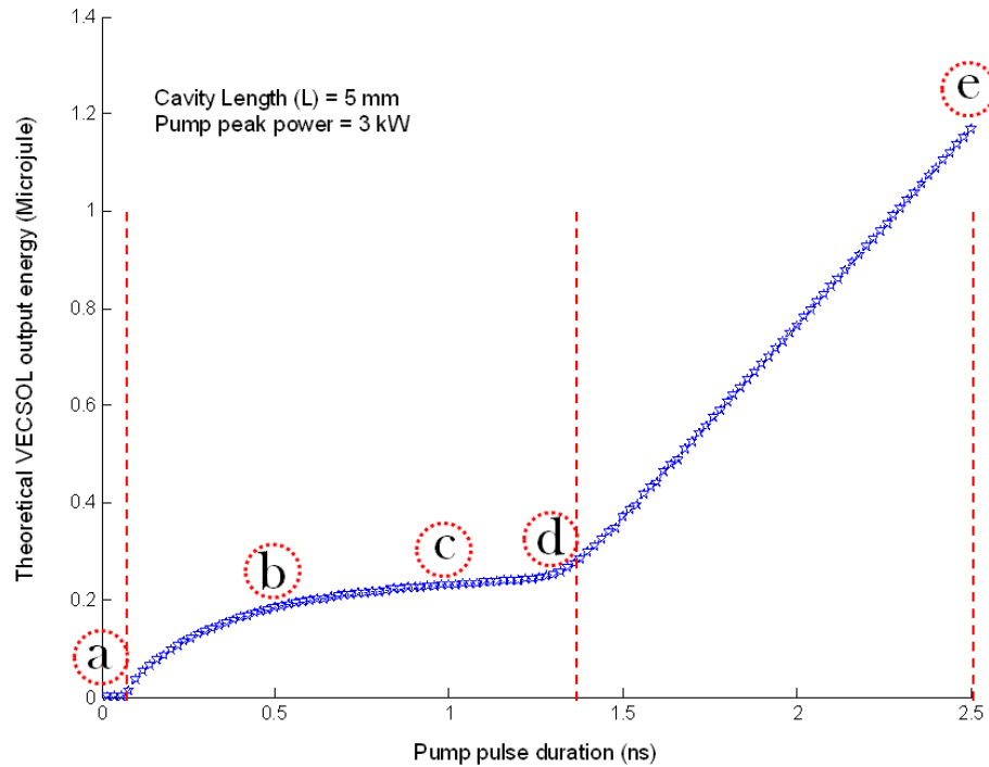
Figure 3.31 – Evolution of the VECSEL output energy versus pump pulse duration.
