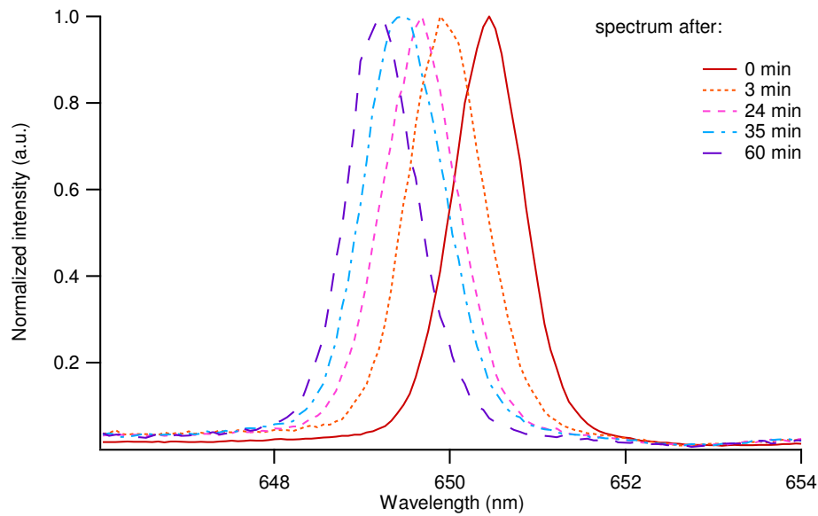
Figure 3.53 - VECSEL red emission spectral blueshift observed and demonstrated for one of the peaks within the multimode emission spectrum as a result of induced refractive index modification caused by photodegradation of the organic gain medium.
