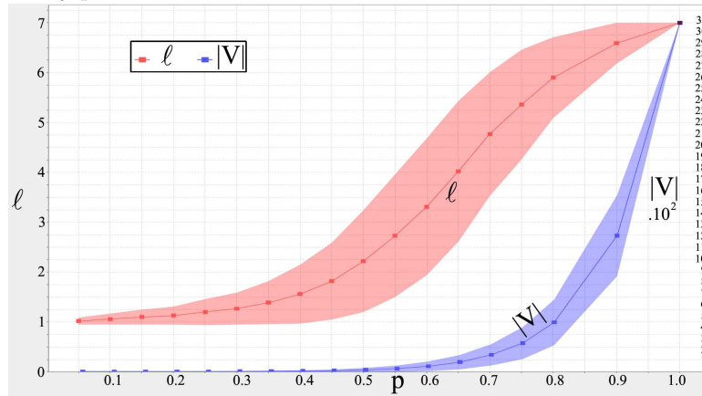
Fig. 7. The average path length has a slow growth compared to the number of nodes, as in BZRG_p . We show the values averaged across simulations and the standard deviation. Color online.
