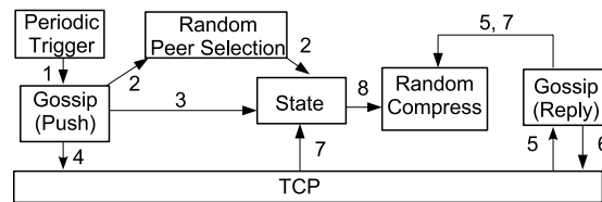
Figure 4.9: Component realisation of RPS [Lin et al. (2011)]
