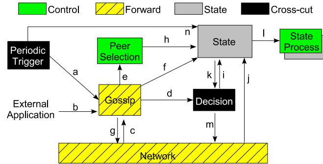
Figure 4.3: GOSSIPKIT’s common architectural pattern (from [Lin (2010)])
