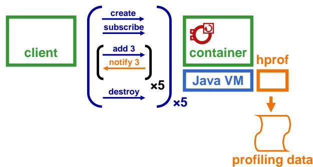
Figure 5.2: Workload of the sample-based profiling campaign
