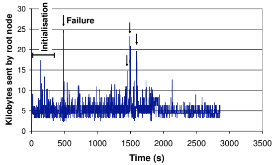
Figure 3.10: SONAR/TCP network usage at the root node on PlanetLab.
